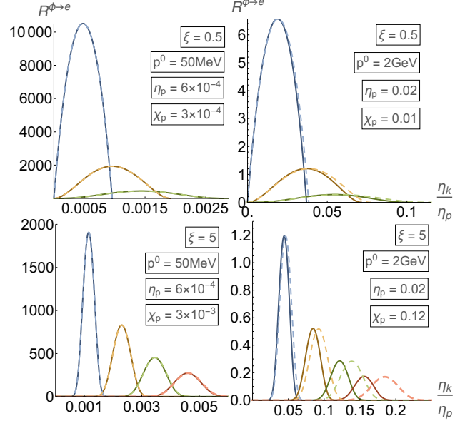
FIG. 1. Here we compare the classical (dashed) and quantum (solid) spectra for scalar emission for a head-on collision of electron and laser-background, with m_\phi = 1 meV, \boldsymbol{\kappa}^0 = 1.55 eV and g_{\phi e} = 1 . In the first row the harmonics s = 1, 2, 3 are shown and in the second row: s = 50, 100, 150, 200 . (In comparison, tail-on collisions have \eta_p \leq \boldsymbol{\kappa}^0 p^0/m^2 \approx 3 \times 10^{-6} .)
