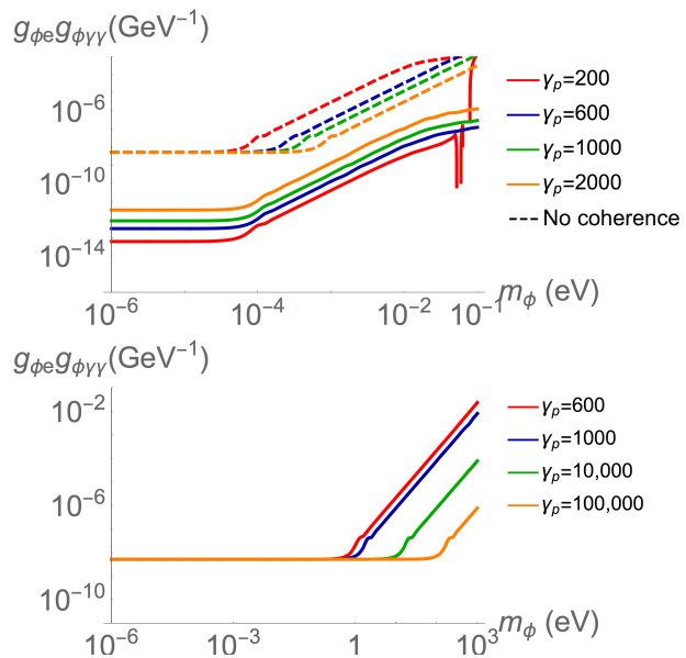
FIG. 6. Projected exclusion bounds from the proposed experimental set-up with tail-on (top) and head-on (bottom) collisions between the electron bunch and laser pulse with an ALPS I-like detection region. The regions above the lines would be excluded, and the coherence effects are only relevant for the tail-on collisions.
