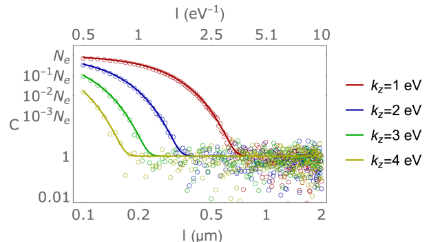
FIG. 3. The coherence changes as one varies the bunch length of a Gaussian-shaped bunch of 10^5 electrons, where |\tilde{j}(k)|^2 = \mathcal{C}N_e |\tilde{j}_{1e}(k)|^2 . The empty circles are the numbers generated from the random Gaussian distribution, and the solid lines are given by the approximating function \mathcal{C}_* .
