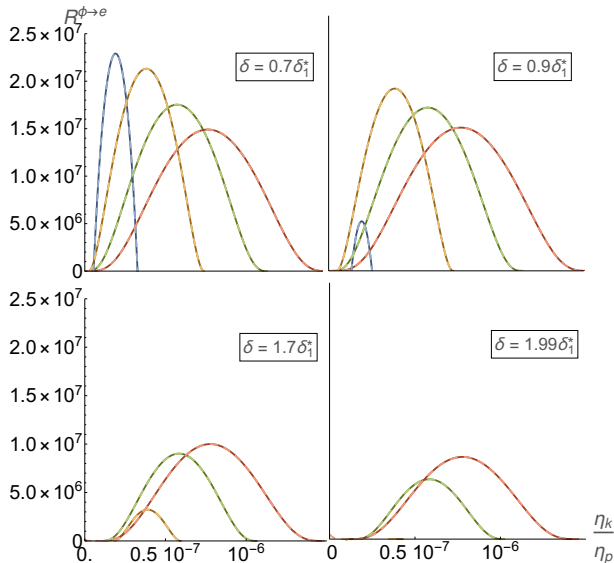
FIG. 2. The classical (dashed) and quantum (solid) spectra for a head-on collision of the laser background with \xi = 10 , \varkappa^0 = 1.55 eV and an initial electron of energy of p^0 = 1.6 MeV ( \approx 2 \times 10^{-5} ). For these parameters, \delta_1^* = 1 eV. As the scalar mass is increased, the first and second harmonics are seen to disappear (each plot has the same axis scale).
