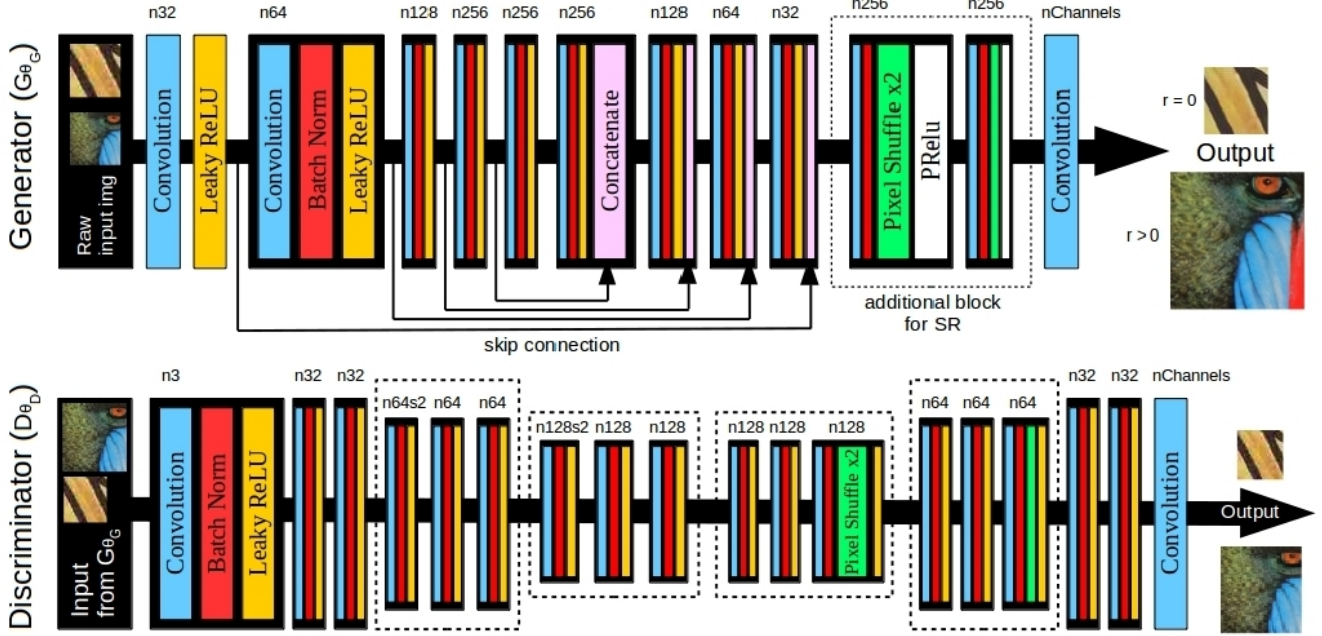
Figure 2. The overall architecture of our proposed network. The convolution layers of the generator have a kernel size 3 \times 3 and stride is 1. Number of filters for each layer is indicated in the illustration, e.g., n32 refers to 32 filters. For the discriminator network, the stride is 1 except for the layers which indicates that the stride is 2, e.g., n64s2 refers to 64 filters and stride=2
