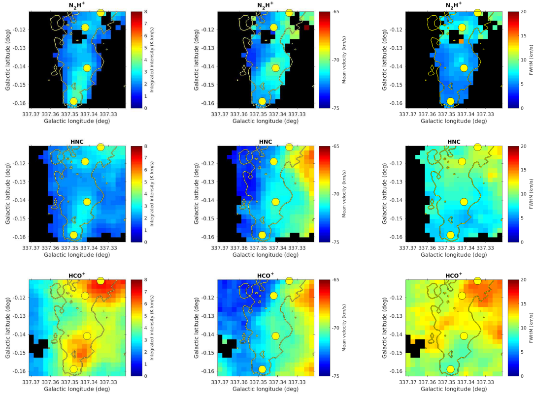
Figure 6. Maps of the N_2H^+ (1–0), HNC (1–0), and HCO^+ (1–0) emission from G337.342–0.119, showing (left) the integrated intensity, (middle) the LSR velocity in \text{km s}^{-1} , and (right) the linewidth \Delta V in \text{km s}^{-1} of the molecular line emission. Pixels with a signal-to-noise ratio less than 10 in the integrated intensity are colored black. The x-axis is Galactic longitude in degrees and the y-axis Galactic latitude in degrees. The yellow circles indicate the positions of the four ATLASGAL clumps comprising the “Pebble.” The contours represent the ATLASGAL emission at a flux level of 0.2 Jy. The lack of large gradients or spatial discontinuities suggest that G337.342–0.119 is a single cloud and not the chance superposition of unrelated clouds.
