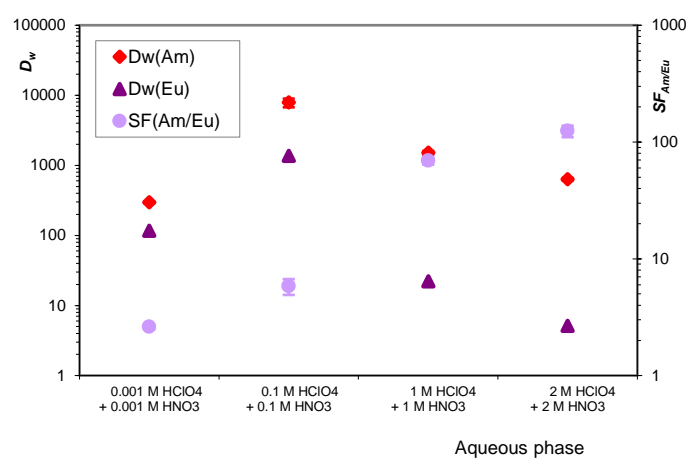
Figure 6. Extraction of Am(III) and Eu(III) by CyMe 4 -BTPhen-functionalized SiO 2 gel 8 as a function of HClO 4 / HNO 3 concentration. Mass of sorbent: approximately 15 mg, phase volume: 0.6 mL, V/m ratio: ~ 40 mL g -1
