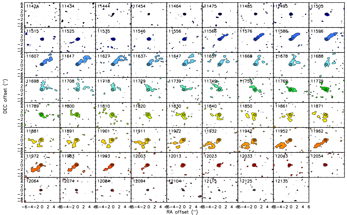
Figure A3. Channel maps for GAMA622429 showing the extended CO emission from this galaxy, across its detected velocity channels. The central velocity is shown top left in each channel map, in \text{km s}^{-1} .
