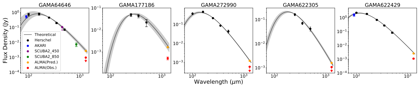
Figure 6. SEDs for our five target galaxies, showing H-ATLAS fluxes from data release 1 (Valiante et al. 2016), AKARI 90 \mu m and SCUBA-2 850 \mu m fluxes where available (see Section 5.2), together with the H-ATLAS temperature fits (including uncertainties in grey) from Agius et al. (2013), assuming \beta = 2 and normalised here to the latest 250 \mu m flux estimates (from Valiante et al. 2016). ALMA predictions for Cycle 3 are shown in orange and ALMA continuum flux observations or 3\sigma upper limits as given in Table 2 are shown in red.
