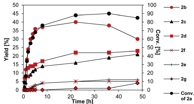
Fig. 3 Aerobic oxidation of lignin model dimer 2a using Au/Li–Al LDH. Conditions: substrate (1 mmol), Au/Li–Al LDH (0.1 g, 1 wt% Au), DPE (10 mL), 120 \text{ }^\circ\text{C} , p = 1 \text{ atm} , O_2 ( 10 \text{ mL min}^{-1} ). All reaction rates were obtained by oxidizing the individual intermediates using the same conditions. For full details refer to ESI (Fig. S5–S7 in ESI†). Conversion and yields were determined by GC–MS using dodecane as internal standard.
