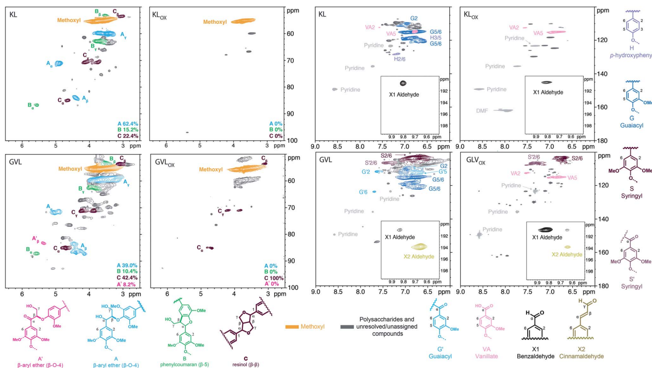
Fig. 4 2D HSQC NMR spectra of KL, KL ox , GVL, and GVL ox lignin. All samples dissolved in 4 : 1 DMSO- d 6 /pyridine- d 5 ; contours color-coded to structures responsible; percentages are determined from volume integrals based on \alpha -C–H with the exception of A' which uses the \beta -C–H signal. The assignment of peaks is based on known lignin spectra and available model compound data.
