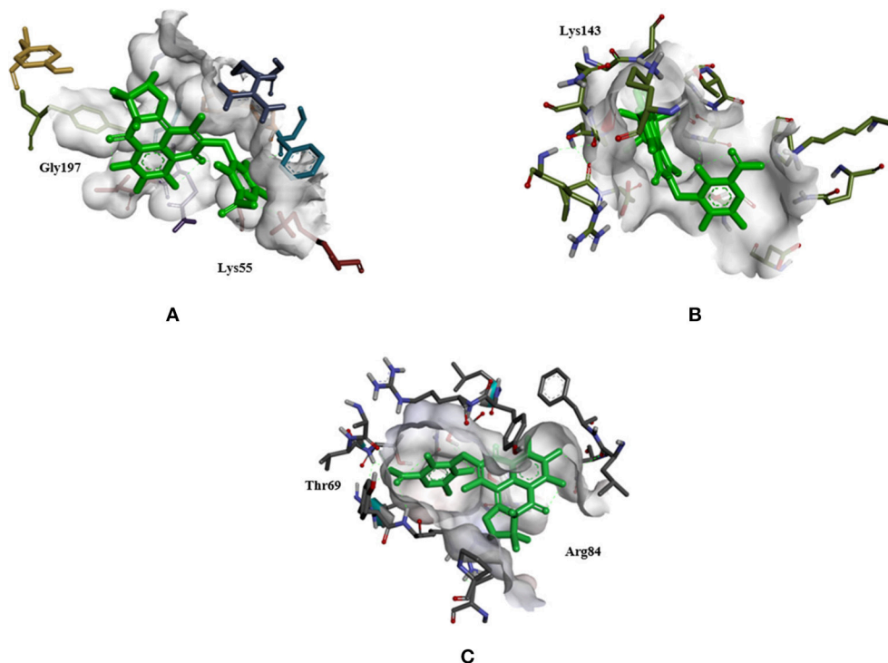
FIGURE 3 | The best docked complex of DnaK, SicA, and SigE with XR770, a histidine kinase inhibitor. (A) DnaK with XR770, interacts with -8.76 binding energy, the target residues being Gly197 and Lys55. (B) SicA with XR770, interacts with -9.78 binding energy, the target residue being Lys143. (C) SigE with XR770, interacts with -11.48 binding energy, the target residues being Thr69 and Arg84.
