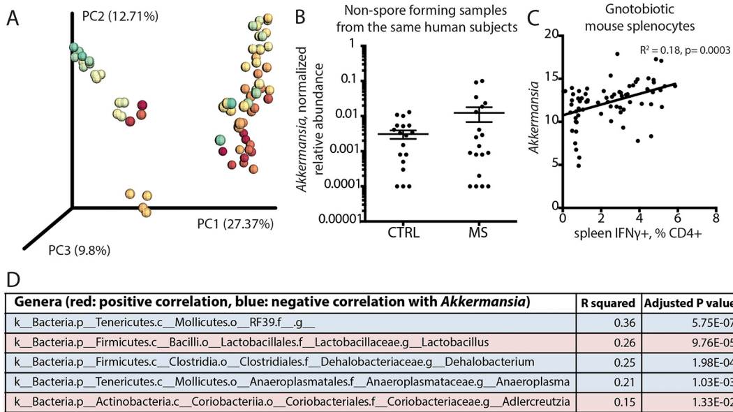
FIG 4 Increased Akkermansia is linked with MS-associated changes in spore-forming bacteria and proinflammatory T lymphocytes. (A) Principal coordinate plot of beta diversity (PCoA; unweighted UniFrac) of mouse fecal microbiota excluding Akkermansia at 2 weeks of colonization with spore-forming bacteria, 2 separate experiments, colored by Akkermansia presence (red to green: low to high). P < 0.001 , significant contribution of Akkermansia presence to determining distance variation (Adonis method for continuous variables). (B) Relative abundance of Akkermansia in controls and MS patients used for isolation of spore-forming bacteria. P = 1.5E-09 , negative binomial Wald test, Benjamini-Hochberg correction for multiple comparisons (across all 144 species detected in the data set). (C) Linear correlation of relative abundance of Akkermansia with IFN- \gamma^+ Th1 lymphocyte differentiation in spleens of mice colonized with spore-forming bacteria. R^2 = 0.18 , P = 0.0003 . (D) Bacterial genera significantly correlated with Akkermansia in vivo .
