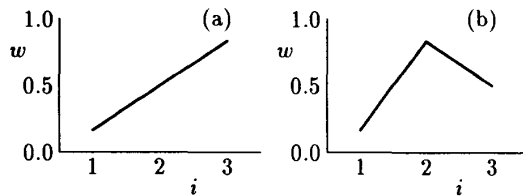
Figure 1: Configurations in a one-dimensional map. (a) Line. (b) Kink.
