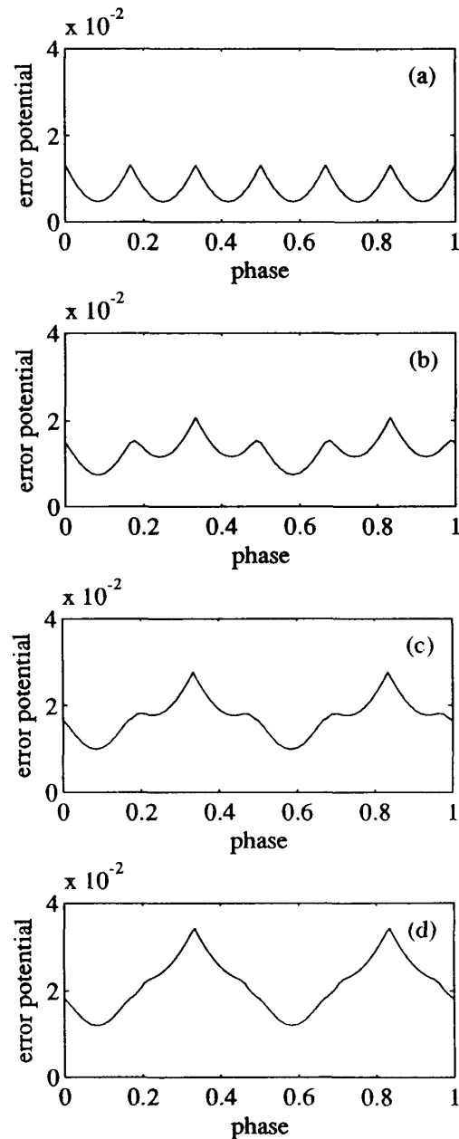
Figure 2: The error potential E as a function of the "phase" \phi/(2\pi) for different values of the interaction strength \sigma . (a) \sigma = 0 . (b) \sigma = 0.04 . (c) \sigma = 0.08 . (d) \sigma = 0.12 .
