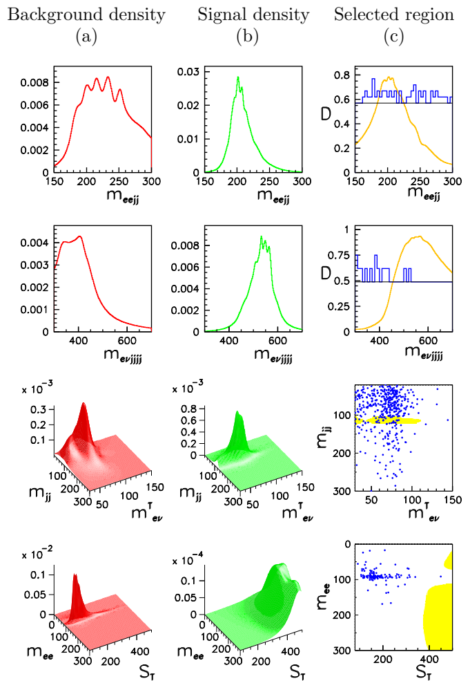
FIG. 2. QUAERO's analysis of signatures involving undiscovered particles. From top to bottom the hypothetical signals are: h_{200} \rightarrow ZZ \rightarrow ee2j , Z'_{550} \rightarrow t\bar{t} \rightarrow e\nu_T 4j , Wh_{115} \rightarrow e\nu_T 2j , and LQ_{225} \rightarrow ee2j . Plots (c) of the first two rows show the discriminant D (curve), the threshold D_{\text{cut}} (horizontal line), and the data (histogram); the region with D > D_{\text{cut}} is selected.
