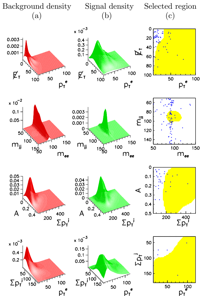
FIG. 1. The background density (a), signal density (b), and selected region (shaded) (c) determined by QUAERO for the standard model processes discussed in the text. From top to bottom the signals are: WW \rightarrow e\mu\nu_T , ZZ \rightarrow ee2j , t\bar{t} \rightarrow e\nu_T 4j , and t\bar{t} \rightarrow e\mu\nu_T 2j . The dots in the plots of the rightmost column represent events observed in the data.
