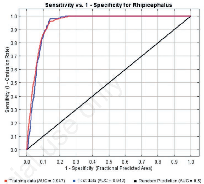
Figure 2. The ROC curve for training data. AUC, Area under the curve; ROC, Receiver operating characteristic.
