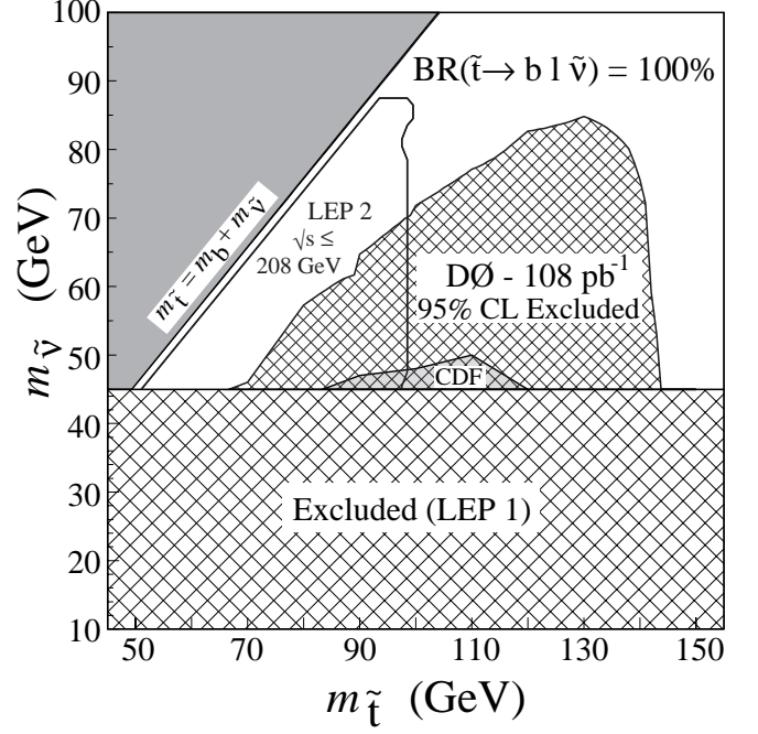
FIG. 4. Excluded regions in the (m_{\tilde{t}}, m_{\tilde{\nu}}) plane for the \tilde{t} \rightarrow b l \tilde{\nu} decay channel in the MSSM. The results of this analysis (labelled D\O 108 \text{ pb}^{-1} ) are compared to the exclusion limits obtained in the \tilde{t} \rightarrow b l \tilde{\nu} decay channel at the Tevatron (CDF), and at LEP 2. Also shown is the sneutrino mass limit obtained at LEP 1.
