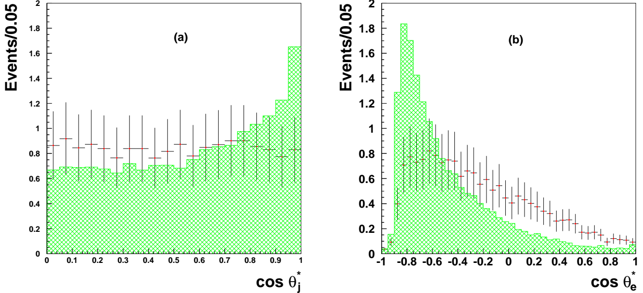
FIG. 8. Distribution of (a) \cos\theta_j^* and (b) \cos\theta_e^* for signal (hatched histogram) and t\bar{t} events (points). The signal was generated at m_0 = 170 GeV, m_{1/2} = 58 GeV, and \tan\beta = 3 . We have multiplied the expected number of signal events (18.5) by a factor of 0.91 to normalize it to the number of t\bar{t} events expected in our base sample.
