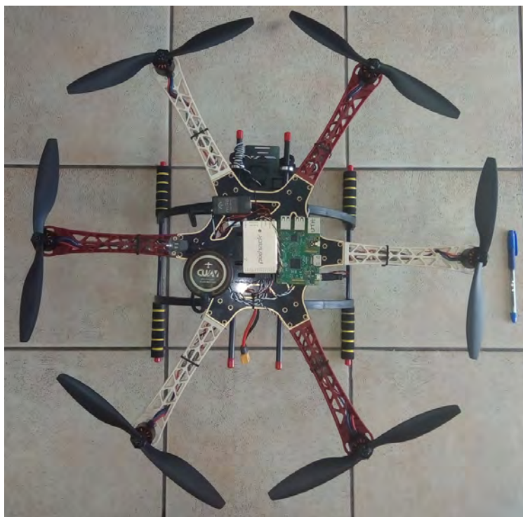
Figure 7.8: Hexacopter.
