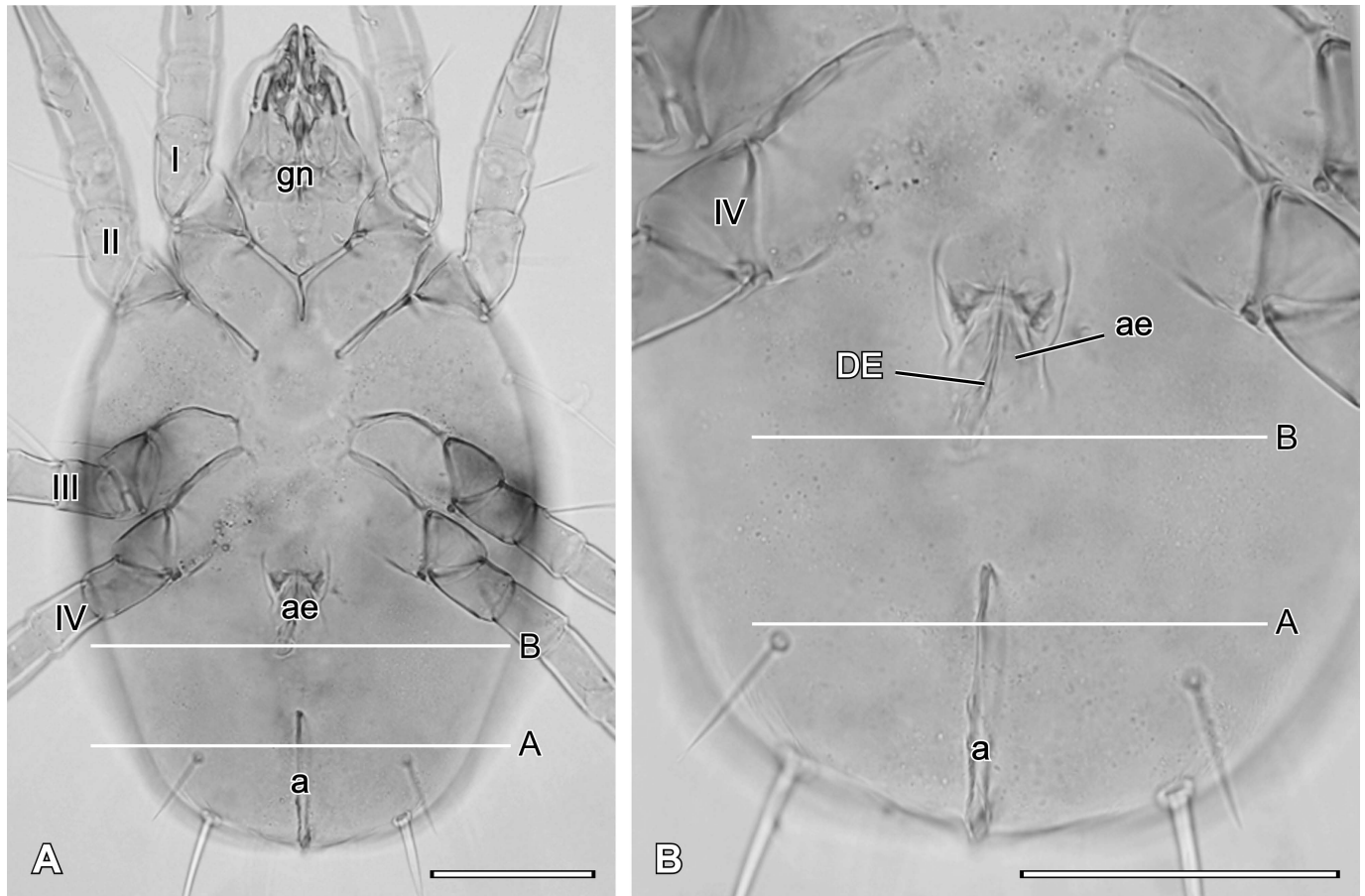
Figure 6 Light microscopic images of Chaetodactylus osmiae male. Male in ventral view (A) and the rear part of idiosoma (B). Scale bars: 0.1 mm. Abbreviations: I-IV – legs I-IV; lines A and B – levels of cross-sections in Figure 7; a – anal slit; ae – aedeagus; DE – ejaculatory duct; gn – gnathosoma.
