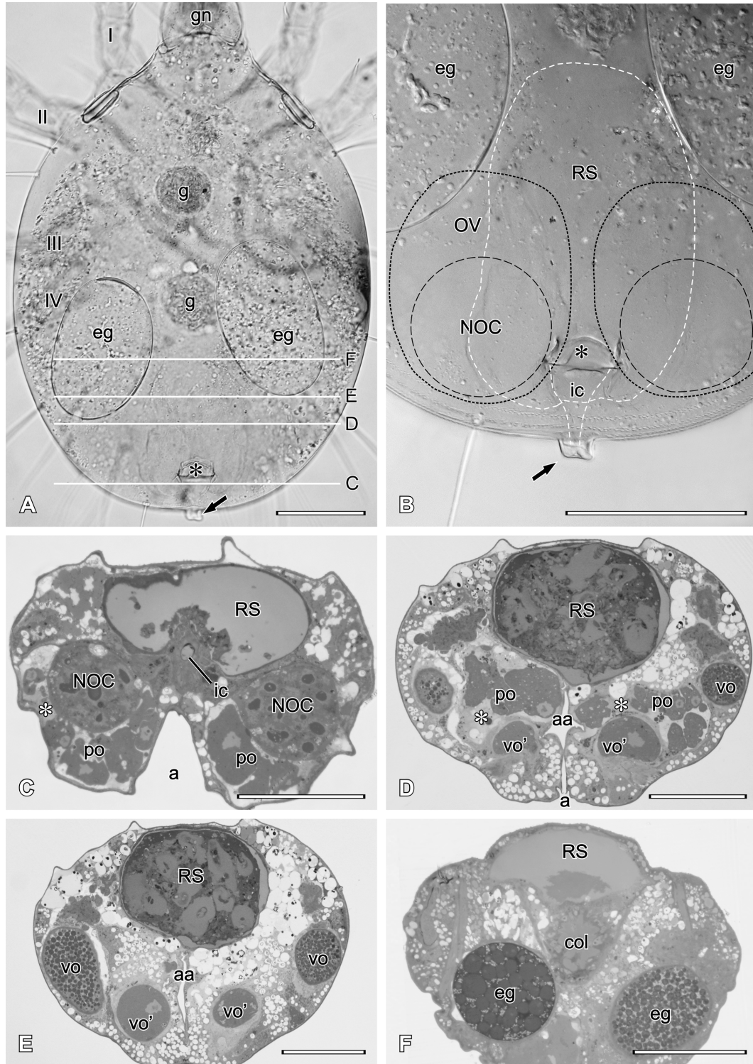
Figure 1 Light microscopic images of a Chaetodactylus osmiae female. Female in dorsal view (A) and the rear part of the idiosoma (B) with marked position of ovaries (OV), nutritive ovarian cells (NOC), spermatheca ( receptaculum seminis ) (RS) and inseminatory canal (ic). C-F – Semithin cross sections of idiosoma marked approx. at levels on (A). Note the spherical shape of nutritive cells (NOC) and irregular, wrinkled outline of previtellogenic oocytes (po) (C, D). Early vitellogenic oocytes (vo') located in the backward running oviduct are spherical (D, E). More developed vitellogenic oocytes (vo) and eggs (eg) in the forward running oviducts show increasing yolk filling (D-F). In the central part of the spermatheca, sperm-containing material delivered by a male is present (D, E), whereas the posterior-most and the anterior part of the spermatheca are free of such material (C, F). Sperm-containing material also shows large, oval structures of medium density (D, E).. Scale bars: 0.1 mm.
