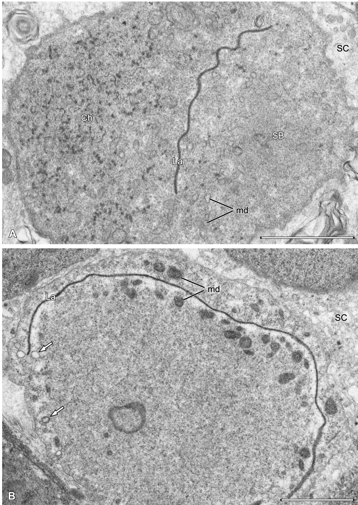
Figure 12 Chaetodactylus osmiae male. TEM. Two consecutive steps in spermiogenesis showing spermatid just after lamella (La) formation (A) and subsequently (B) when multiform dense mitochondrial derivatives (md) appear along the lamella. In (A) the spermatid is sectioned through the lamella (La), separating chromatin threads (Ch) and organizing the spongy body (SB). In (B) the spermatid section shows the lamella (La) flanked by dense and multiform mitochondrial derivatives (md). Several small vesicular mitochondrial derivatives can be seen (arrows) close to the left end of the lamella. Scale bars: 2 \mu m. Other abbreviations: SC – stroma cell.
