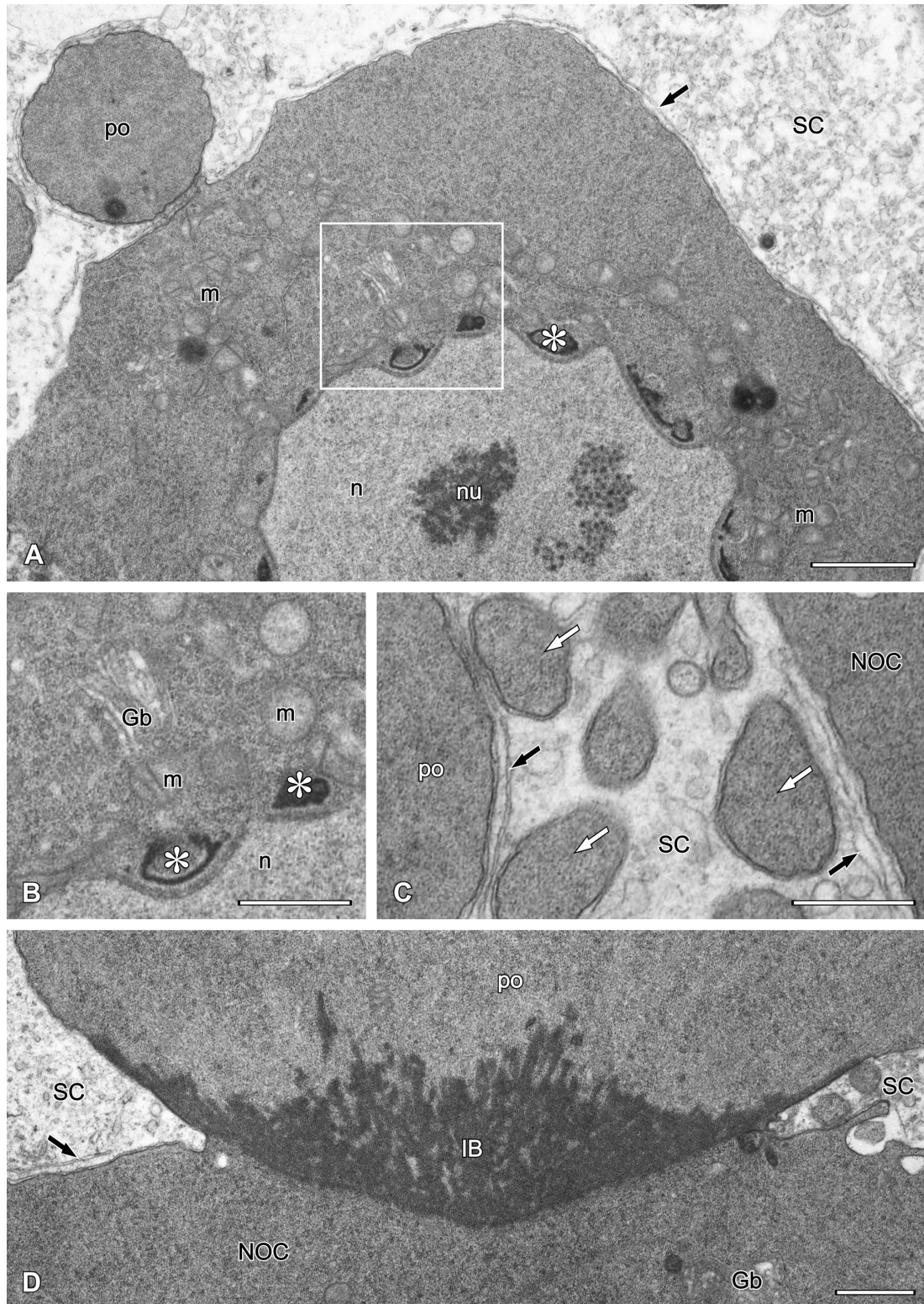
Figure 4 Chaetodactylus osmiae female. TEM. (A) Advanced previtellogenic oocyte showing nucleus (n) with nucleolus (nu). The nuclear envelope has concavities in sites rich in pores, with adhering nuage material (asterisk). Mitochondria (m) are grouped around the nucleus. Another oocyte sectioned tangentially (po) is also present. In the stroma cell (SC), an arrow marks a conspicuous ER cisterna. (B) Enlarged fragment of the oocyte marked in (A): note nucleus (n), a Golgi body (Gb), nuage (asterisks) and mitochondria (m). Note the different appearance of nuage material which is not granular as in the nutritive cell and early oocytes (compare with 2B and 3A-B).. (C) A gap between a nutritive cell (NOC) and previtellogenic oocyte (po) filled with a stroma cell (SC) in which several nutritive cell protrusions (white arrows) are embedded. ER cisterns in the stroma cell are also present (black arrows). (D) Intercellular bridge (IB) connecting a nutritive cell (NOC) and previtellogenic oocyte (po), filled with electron-dense granular material in fan-like arrangement. Golgi body (Gb) in nutritive cell and ER cisterna (arrow) in stroma cell (SC) are marked. Scale bars: A – 2 \mu\text{m} , B-D – 1 \mu\text{m} .
