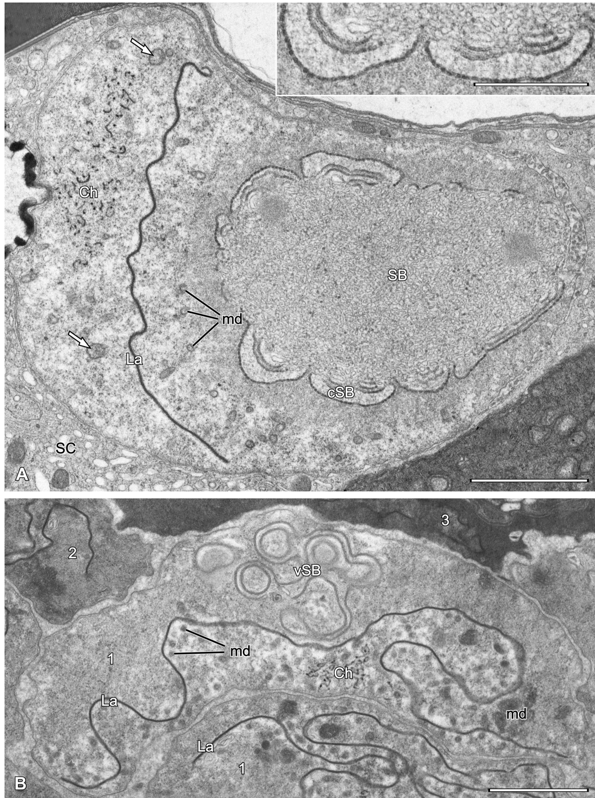
Figure 13 Chaetodactylus osmiae male. TEM. (A) Late spermatid showing chromatin threads (Ch), dense lamella (La) and elaborate spongy body (SB). Small vesicles of mitochondrial derivatives (md) are present around the spongy body and along the dense lamella; however, larger and more electron-dense mitochondrial derivatives are also present (arrows). Anastomosing tubules of the spongy body are encircled by characteristic arcuate cisterns (cSB) formed by double membranes similar to annulate lamellae. (Inset) Arcuate cisterns and tubules of spongy body under higher magnification. (B) Two very late spermatids not yet condensed (1) and fragments of finally condensed spermatids (2,3). Each spermatid contains one meandering dense lamella (La) which separates chromatin threads (Ch) from double membrane vesicles (vSB) putatively derived from arcuate cisterns (cSB in A) surrounding the spongy body. Multiformal mitochondrial derivatives (md) are frequently located along dense lamella. Scale bars: A,B – 2 \mu m, A inset – 1 \mu m. Other abbreviations: SC – stroma cell.
