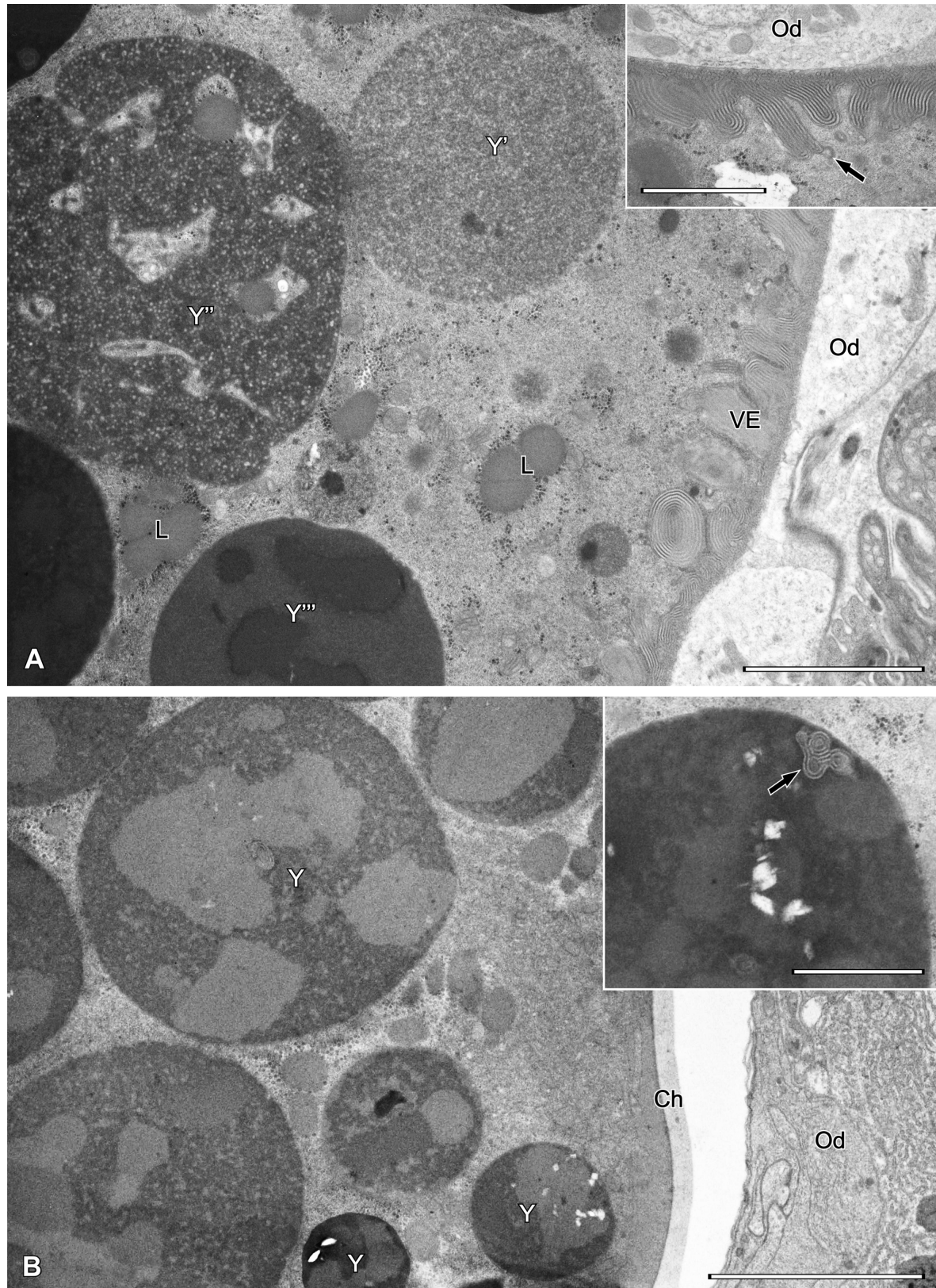
Figure 5 Chaetodactylus osmiae female. TEM. (A) Vitellogenic oocyte in upper (forward-running) part of oviduct (Od), containing yolk spheres in subsequent stages of development ( Y' , Y'' and Y''' ) and lipid droplets (L) surrounded by glycogen. Lamellar vitelline envelope (VE) covers the surface of the oocyte. Inset: Higher magnification of vitelline envelope adhering to oviduct (Od). Vesicle delivering vitelline envelope material from Golgi body is indicated by an arrow. (B) More advanced vitellogenic oocyte covered with thin and homogeneous chorion (Ch) in the upper oviduct (Od). Yolk (Y) spheres of two types, larger and less dense and smaller and more dense, containing crystalline electron-lucid inclusions. Inset: Yolk sphere with electron-lucid inclusions and meandering structure (arrow). Scale bars: A,B – 5 \mu\text{m} , A inset, B inset – 2 \mu\text{m} .
