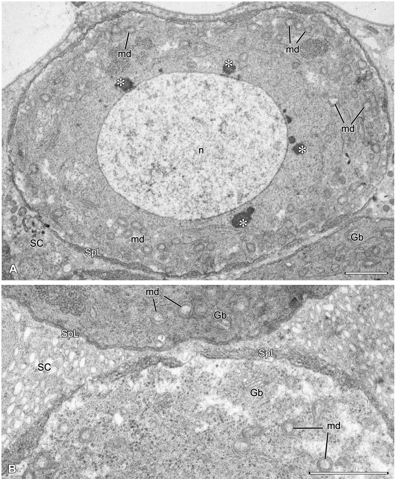
Figure 10 Chaetodactylus osmiae male. TEM. (A) Spermatocyte more advanced than those in Figure 9B, embedded in stroma cell (SC). Note thicker spongy layer (SpL) covering the cell surface, large nucleus (n) and nuage material (asterisks). Peripheral cytoplasm contains many mitochondrial derivatives (md): they are roundish and possess one circular crista. A Golgi body (Gb) is present under the spongy layer of a neighboring spermatocyte (right bottom). (B) Peripheral parts of two spermatocytes separated by a stroma cell (SC). Compare the thickness of the spongy layer (SpL) in the upper, less advanced spermatocyte and that of the lower, more advanced cell. Both cells have similar Golgi bodies (Gb) and mitochondrial derivatives (md) but the more advanced, lower spermatocyte shows empty spaces in its peripheral cytoplasm. Scale bars: 2 \mu m.
