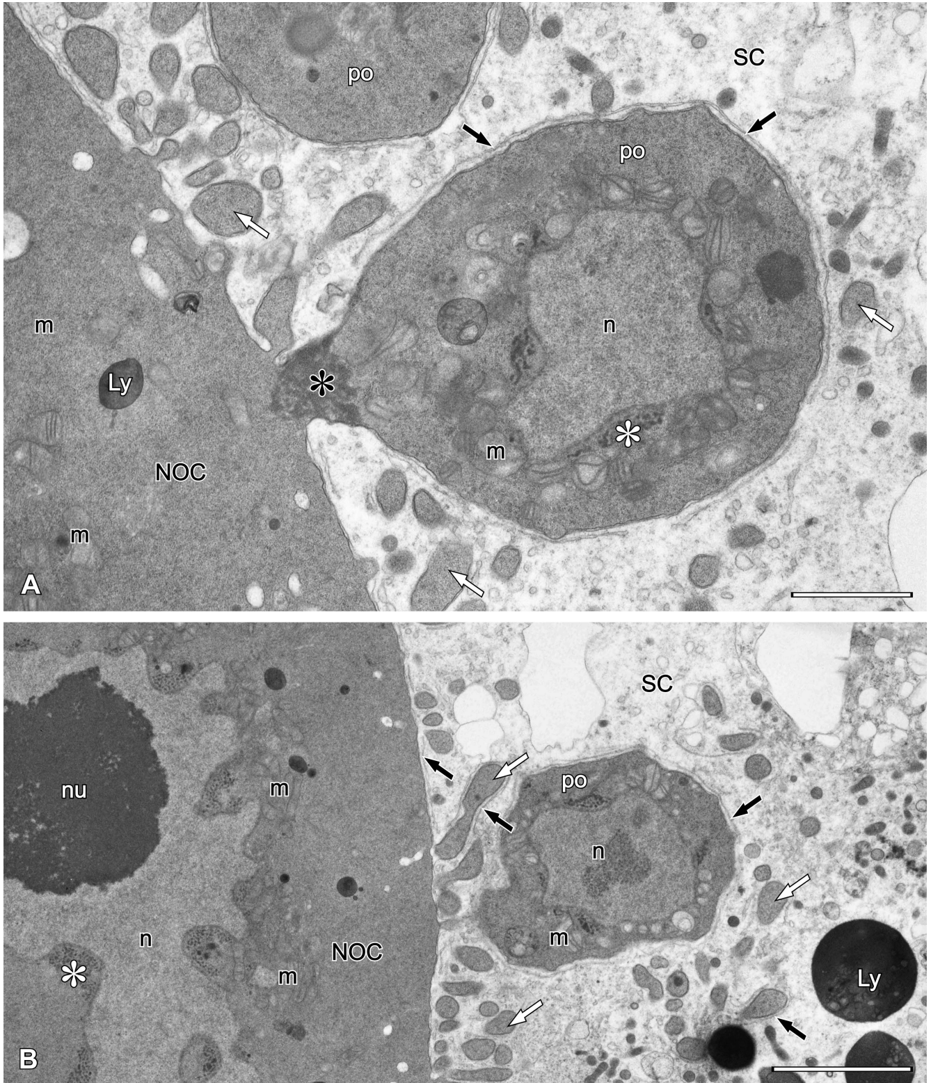
Figure 3 Chaetodactylus osmiae female, two aspects (A, B) of the peripheral part of the nutritive ovarian cell. TEM. (A) Nutritive cell (NOC) shows mitochondria (m) and lysosome (Ly), and is connected via an intercellular bridge (black asterisk) with an early previtellogenic oocyte (po). The other previtellogenic oocyte is partly visible above. The oocyte nucleus (n) is irregular in outline and envelope concavities contain electron dense nuage material (white asterisk). Mitochondria (m) in the oocyte closely surround the nuclear envelope. Somatic stroma cells (SC) show few ribosomes and are penetrated by many protrusions of a nutritive cell (white arrows). Note ER cisterns (black arrows) running in stroma cell parallel to its contacts with germ-line cells (i.e. nutritive cell and oocytes). (B) Another aspect of the nutritive cell periphery similar to (A). Note a lobe of the nucleus (n) with a nucleolus (nu) in the nutritive cell; concavities of the nuclear envelope are filled with nuage material (white asterisk) whereas mitochondria (m) are clustered close to the nucleus in both the nutritive cell and oocyte (po). Nutritive cell protrusions and ER cisternae in stroma cells are indicated by white and black arrows, respectively. Other abbreviations: Ly – lysosome in stroma cell. Scale bars: A – 2 \mu m, B – 5 \mu m.
