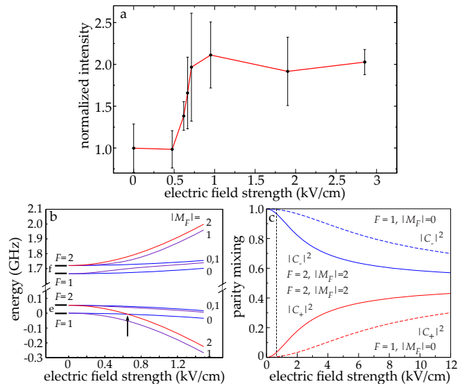
FIG. 9: (Color online): (a) Bias-voltage dependence of the transmission for OH in its hfs {}^2\Pi_{3/2}, v = 0, J = 3/2, e, F = 2 state. In all measurements the same switching sequence is applied and the integrated intensity of the focused molecular packet is plotted against the nominal electric field strength inside the electric field stages. (b) Stark energies of the individual hyperfine states of OH in its {}^2\Pi_{3/2}, v = 0, J = 3/2 rotational state. (c) Parity components of the two hyperfine states that cross at 640 V/cm. See text for details.
