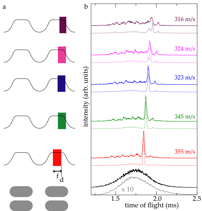
FIG. 8: (Color online) a) Graphical representations of the high-voltage switching parameters d and f . b) Deceleration sequence of OH in its high-field seeking {}^2\Pi_{3/2}, v = 0, J = 3/2, e state, with the simulated time-of-flight profiles underneath the experimental measurements for different focusing and deceleration parameters. The lowest traces are free-flight profiles. The second (red) traces show the arrival-time distribution for focusing at a constant velocity of 355 m/s. The following traces are TOFs for deceleration from 355 m/s to successively slower final velocities, as noted in the graph.
