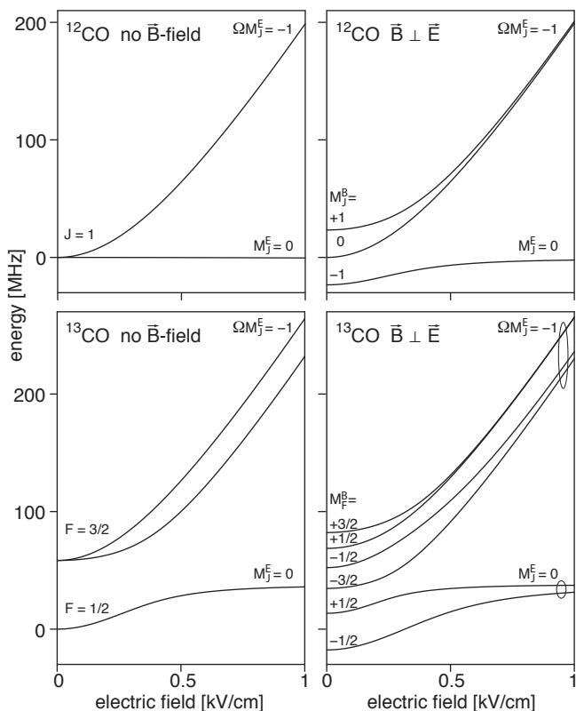
FIG. 4: Energy of the upper (positive parity) \Lambda -doublet component of the J = 1 level of ^{12}\text{CO} (upper panels) and ^{13}\text{CO} (lower panels) in the electronically excited a^3\Pi_1 , v = 0 state as a function of the electric field strength, without (left column) and with (right column) an offset magnetic field. The strength of the magnetic field is 50 Gauss and its direction is perpendicular to the direction of the electric field. The labeling of the energy levels is explained in the text.
