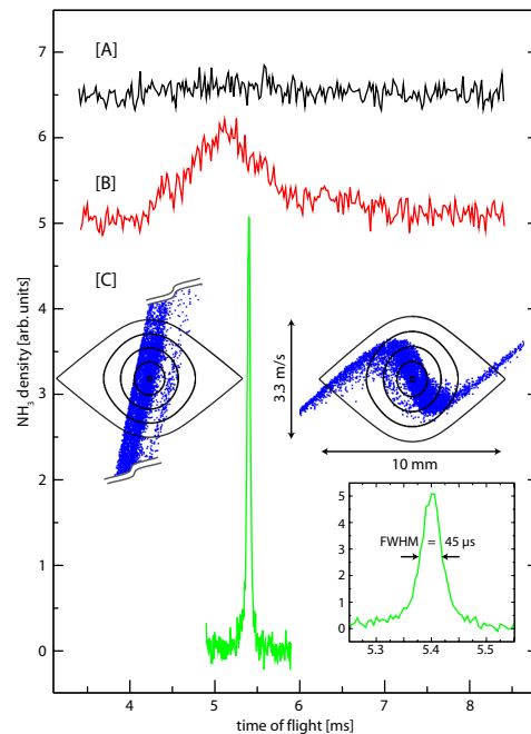
FIG. 2: (Color online) Density of ammonia molecules behind the microwave cavity as a function of time (in milliseconds) without microwaves ([A]), with 3.0 W of microwaves continuously coupled in ([B]) or with pulsed application of the microwaves for two thirds of the time ([C]). The curves are offset for clarity, but all have the same vertical scale. For the measurements in panel [C], the microwaves are applied synchronously with the motion of an ammonia molecule that moves on the molecular beam axis with a forward velocity of 25 m/s. The longitudinal phase space distribution of the molecules at the first time that the microwaves are switched on and at the last time that they are switched off is shown on the left and right side of the peak, respectively, overlaid on the longitudinal phase space acceptance diagram.
