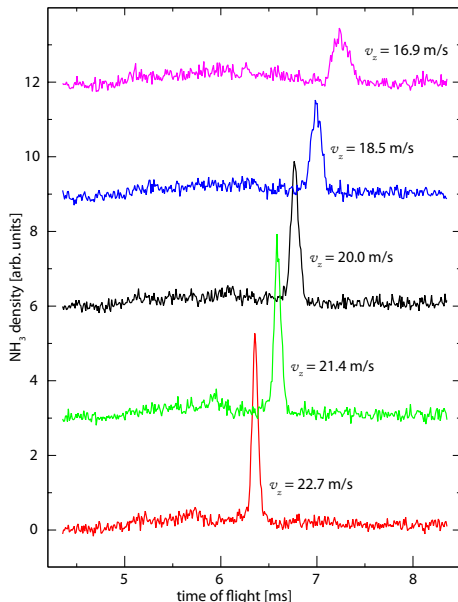
FIG. 3: (Color online) Density of ammonia molecules behind the microwave cavity as a function of time for two different acceleration, a guiding and two deceleration sequences (curves vertically offset for clarity). Ammonia molecules that enter the cavity with v_z=20.0 m/s exit with the indicated velocity.
