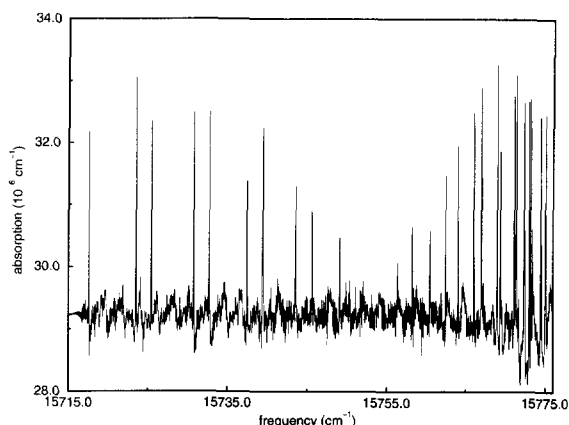
Fig. 2. The absorption spectrum of 365 mbar of 18 O 2 around 635 nm measured via the PS-CRD method. The spectral structure is due to the b 1 Σ g + (v' = 2) ← X 3 Σ g - (v'' = 0) transition.
