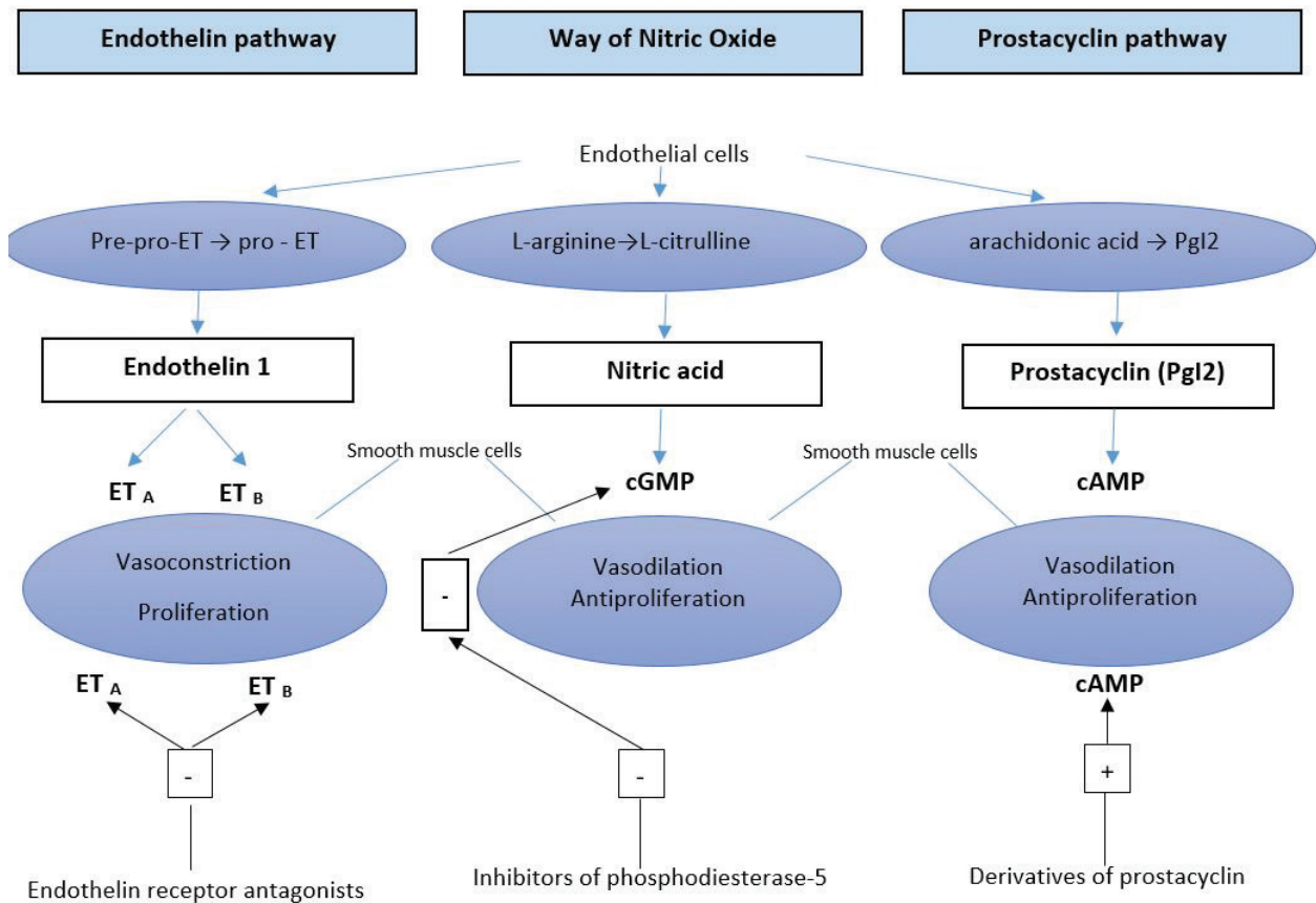
Figure 4. Mechanisms of the pathogenesis of pulmonary hypertension as targets for its pharmacological correction. Note: Pre-pro-ET is an endothelin precursor, ETA is an endothelin type A receptor, an ETB is an endothelin type B receptor, cGMP is a cyclic guanine monophosphate, cAMP is a cyclic adenosine phosphote, Pgl2 is a prostaglandin I2.
