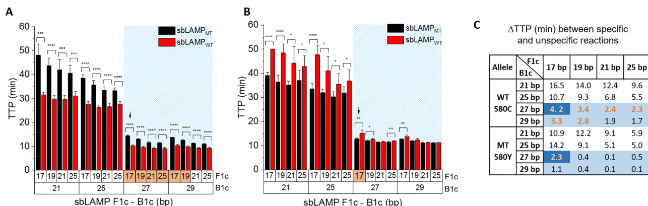
Figure 1. Results of sbLAMP using different F1c-B1c primer lengths. (A) Comparison of WT template ( 580C ) amplification by WT specific (sbLAMP WT ) and MT specific (sbLAMP MT ) primer sets with different lengths of F1c and B1c. (B) Comparison of MT template ( 580Y ) amplification by WT specific (sbLAMP WT ) and MT specific (sbLAMP MT ) primer sets with different lengths of F1c and B1c. (C) Table showing the \Delta TTP values between specific and unspecific primer sets. Average TTP values of specific reactions below 20 min are blue shaded. \Delta TTP values above 2 min are orange colored. Average of two experiments performed in triplicates using 5 \times 10^4 copies/reaction of synthetic DNA. Selected sbLAMP primer sets are indicated with arrows in the plots and dark blue cells in the table.
