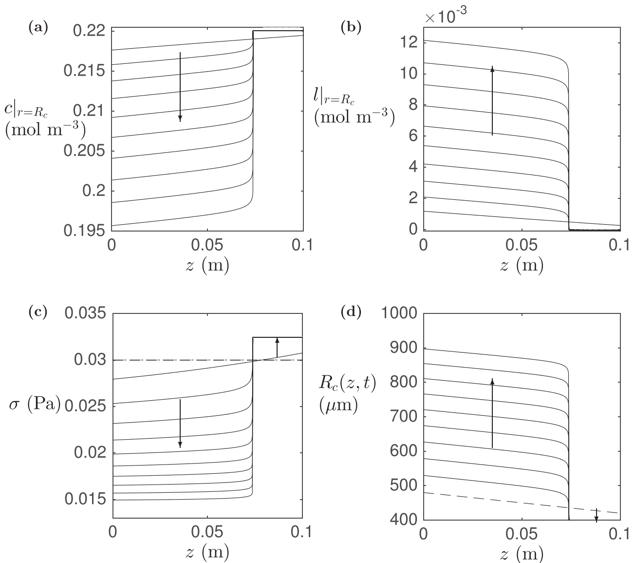
Fig. 6. Evolution of (a) c|_{r=R_c} , (b) l|_{r=R_c} , (c) \sigma|_{r=R_c} and (d) R_c(z, t) for an initially non-uniform layer of rat cardiomyocytes. Cell layer grows outwards at upstream end ( z < 7.36 cm), but recedes to fibre surface in 5 days at downstream end ( z > 7.38 cm) (d) where \sigma > \Sigma_d (c). Note the scales on the axes, from which it can be seen that the gradient of the surface between the regions of growth and recession is of order 1. Initial cell layer outer radius R_{c,init}(z) = (480 - 6.1 \times 10^{-4}z) \mu\text{m} . Mean outer radius at t=60 days, \bar{R}_c = 750 \mu\text{m} . Parameter values as in Fig. 4 ( Q_{l,in} = 3.33 \times 10^{-8} \text{ m}^3 \text{ s}^{-1} , P_{l,out} = 1.965 \times 10^5 \text{ Pa} ). Lines and arrows as in Fig. 4.
