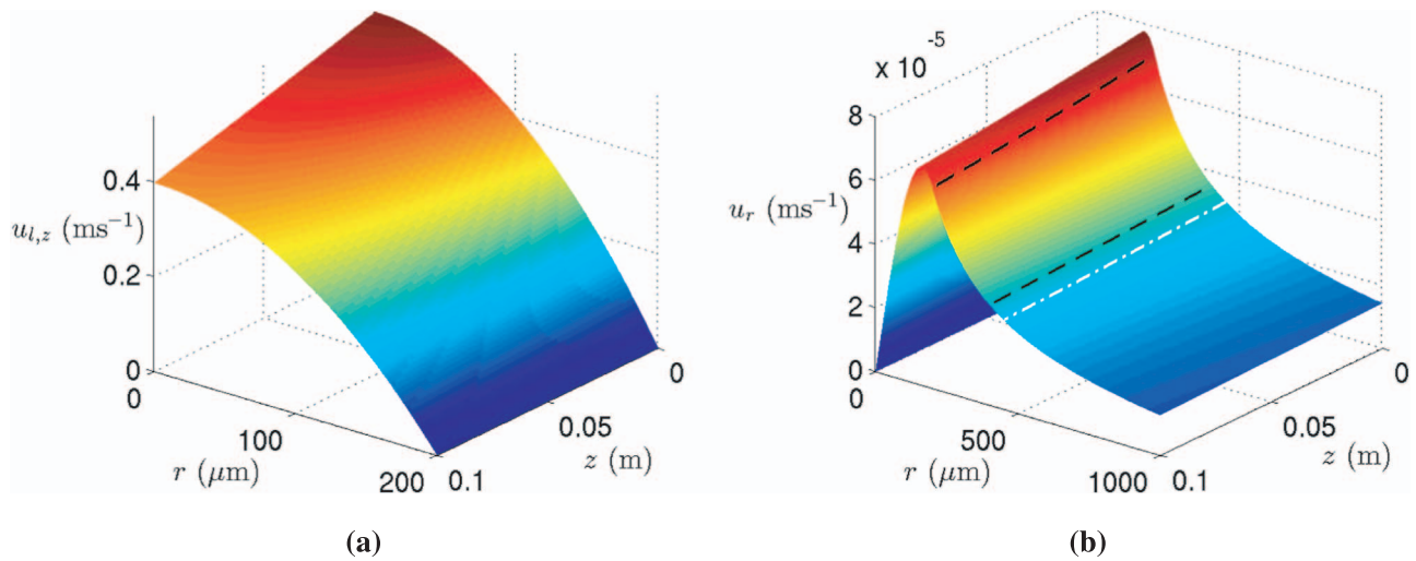
Fig. E2. (a) Lumen axial flow velocity u_{l,z} and (b) radial flow velocity u_r , for the uniform depth cell layer in Fig. E1(a). Profiles for the non-uniform cell layer in Fig. E1(b) are almost identical. All parameter values and dashed lines as in Fig. E1.
