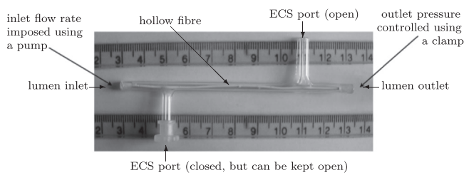
Fig. 1. Photograph of a single-fibre HFB module. ECS=extra-capillary space. Adapted from Shipley and Waters (2012).
