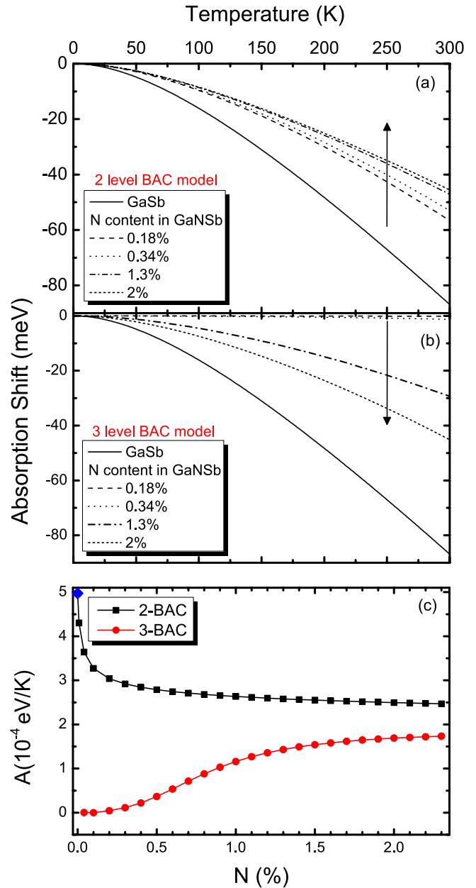
Figure 5. Temperature-dependent energy shift of the absorption edge calculated for \text{GaN}_x\text{Sb}_{1-x} using (a) two level BAC model and (b) three level BAC model. The arrows show the direction of the trend as a function of N contents. (c) Comparison of modeled parameter A as a function of composition, calculated using two level BAC (square) and three level BAC (circle). In the modelling, the parameter B was kept constant and equal to the value of GaSb 184.6 K. The diamond mark at N = 0\% corresponds to the A value of GaSb.
