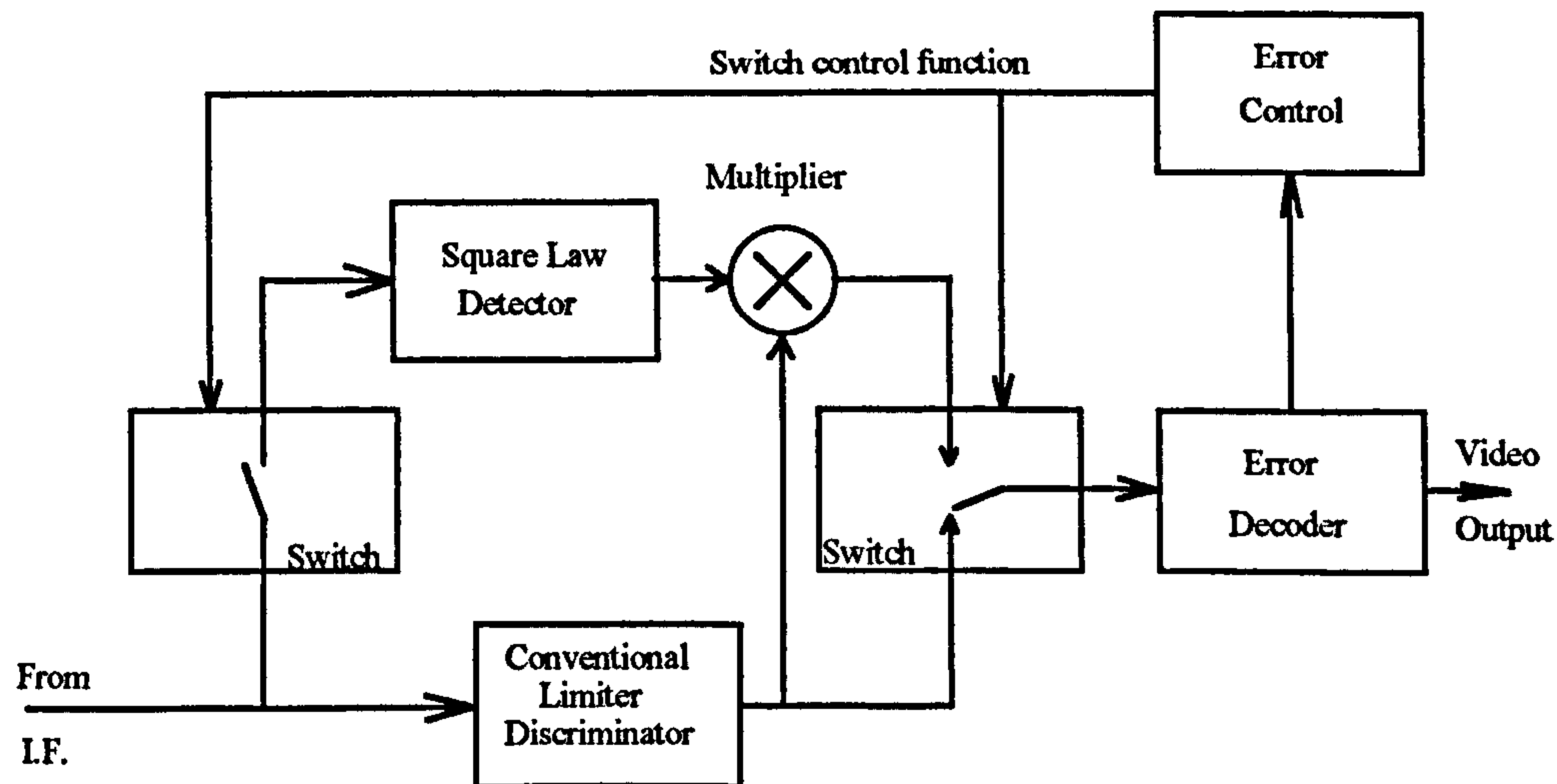
Figure 18/19 Roberts envelope multiplication discriminator implemented as an adaptive error controlled demodulator
