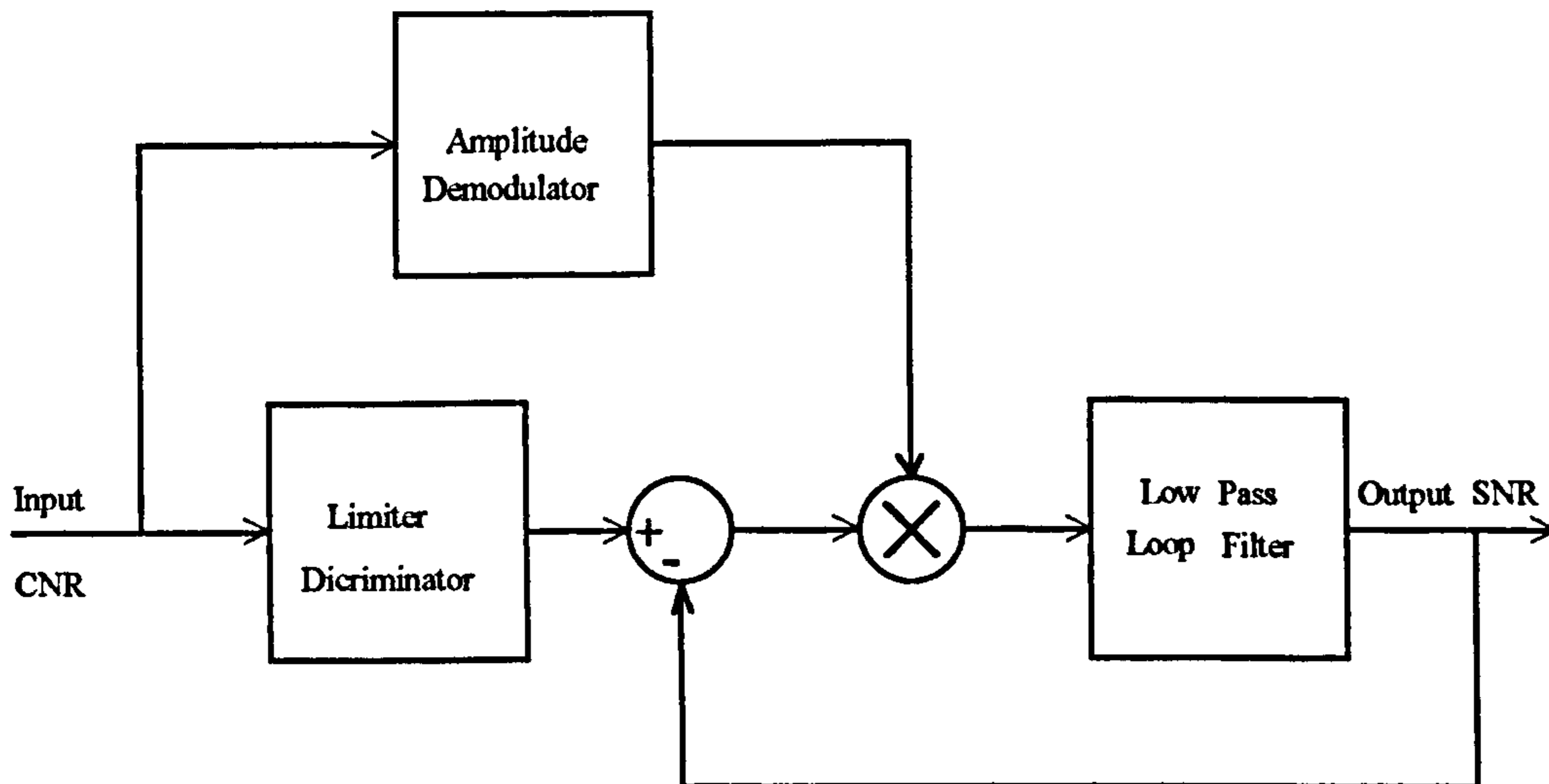
Figure 11/1 Frequency Lock Loop Demodulator (Baseband Version)
