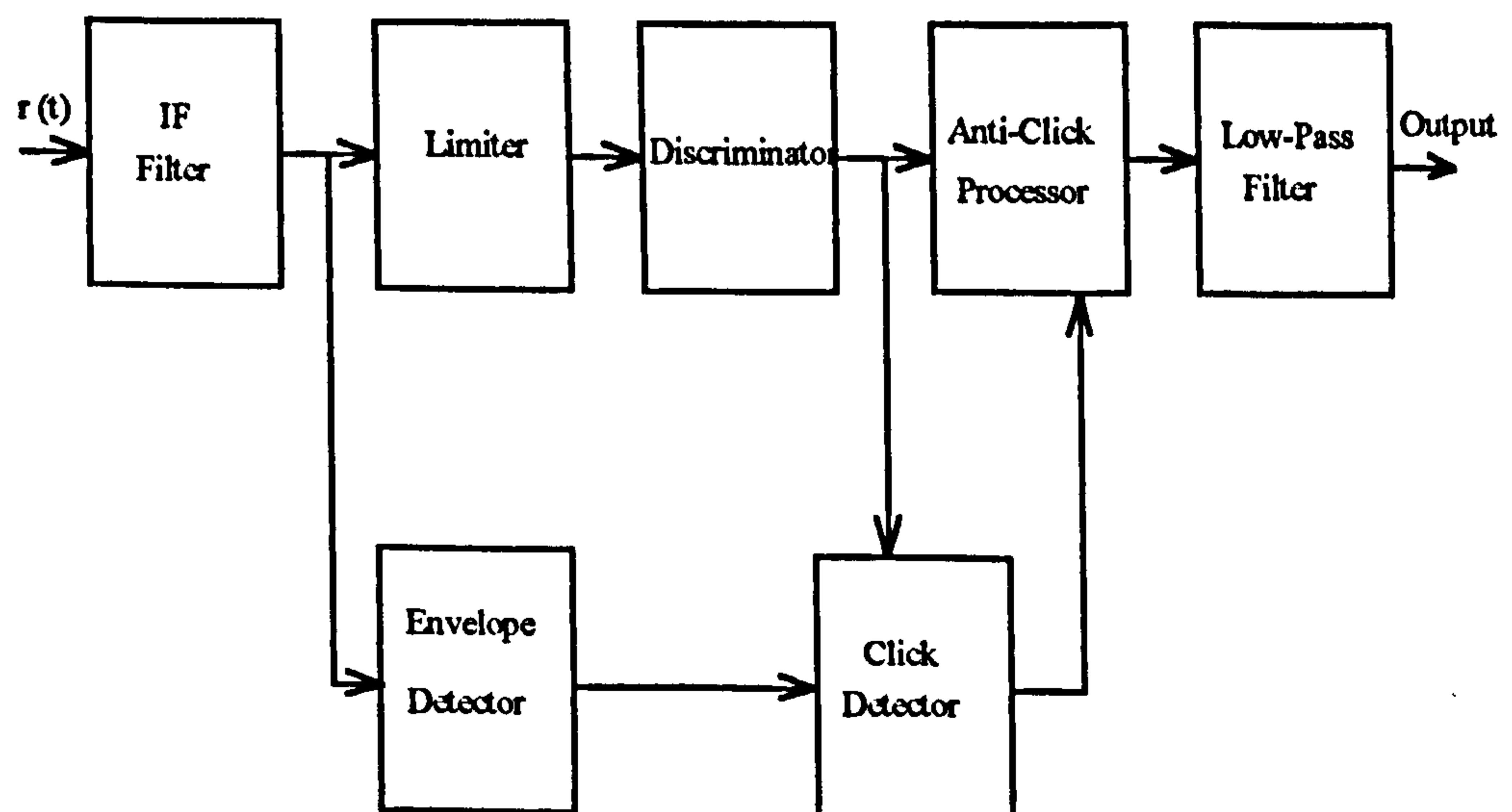
Figure 15/1 FM Demodulator with Click Elimination
