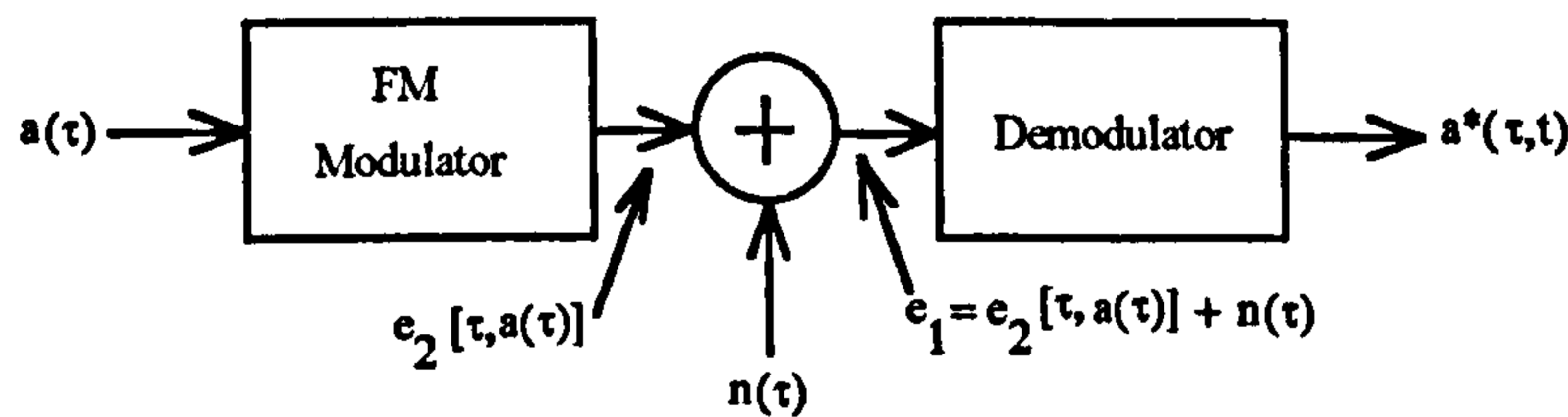
Figure 16/2 Demodulator Model
