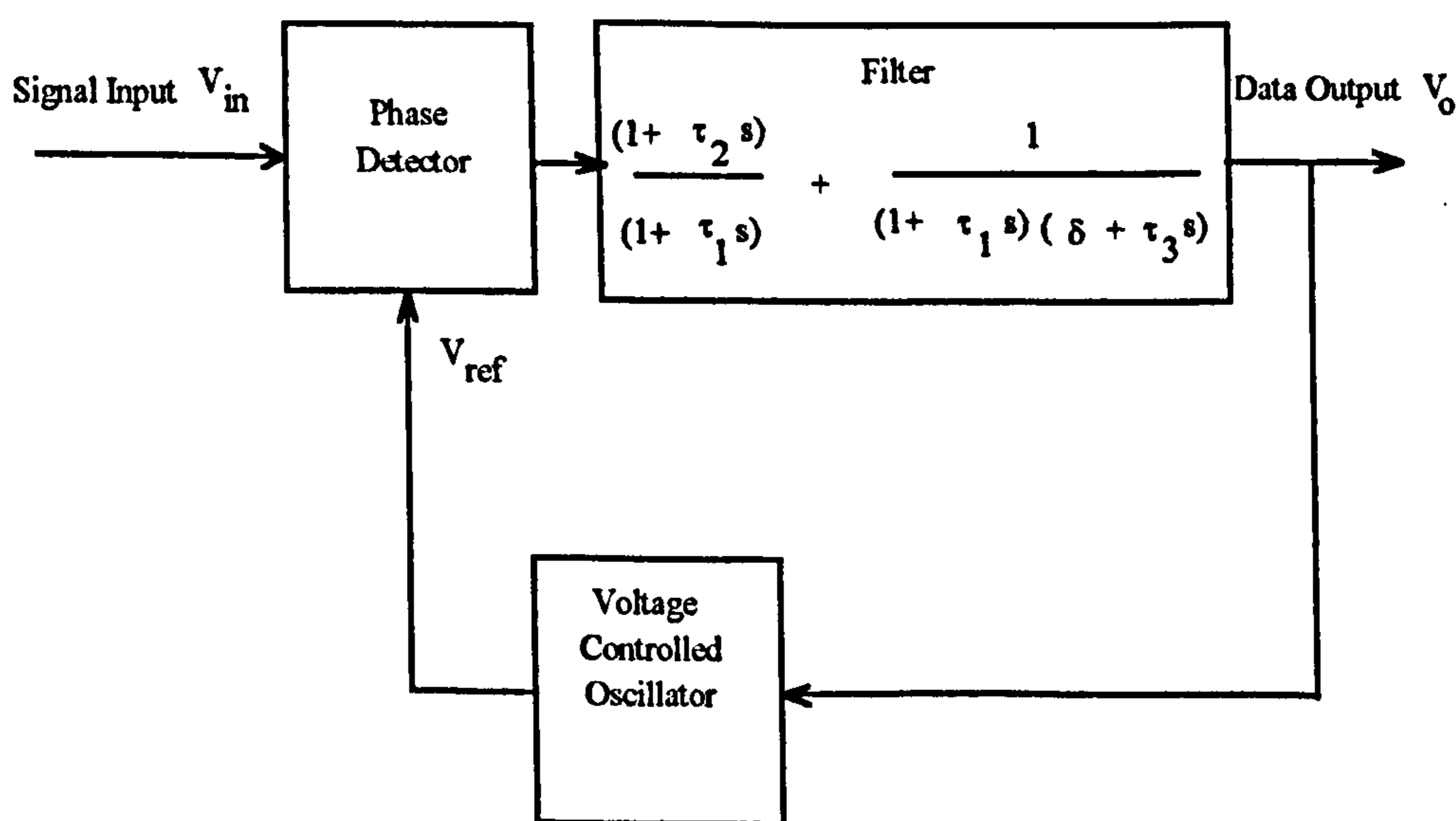
Figure 10/9 Third Order Phase Lock Loop Demodulator (Crow and Tausworthe)
