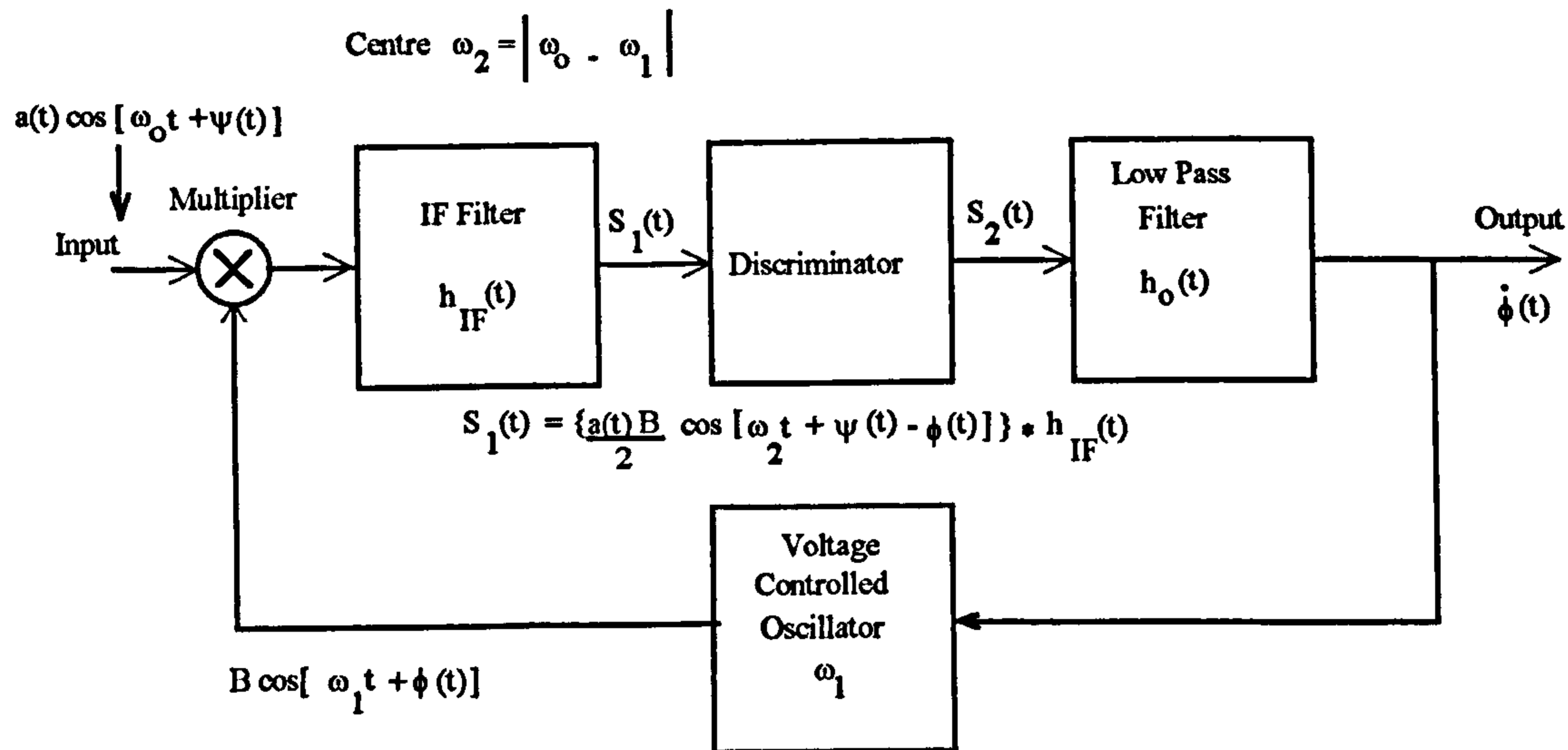
Figure 17/3 Block Diagram Frequency Demodulator with Feedback
