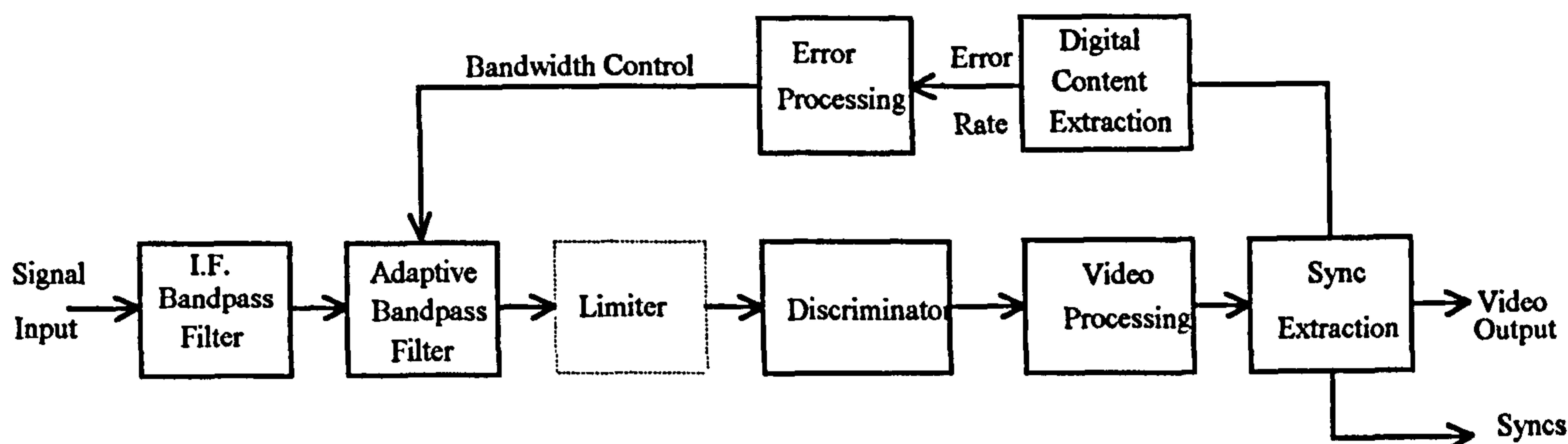
Figure 18/4 Error controlled demodulator concept
