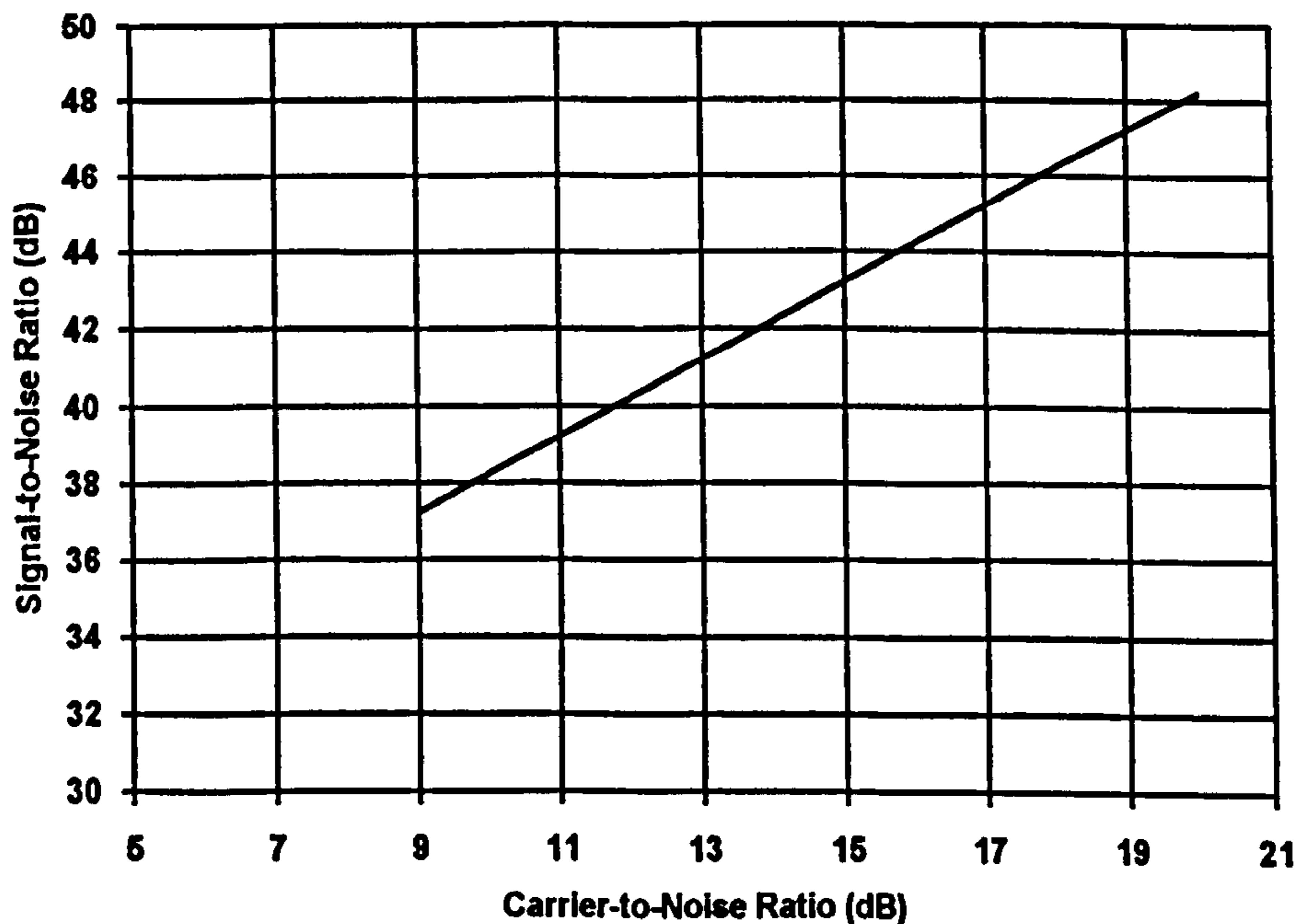
Figure 5/2 - C, D and D2 TV Systems
