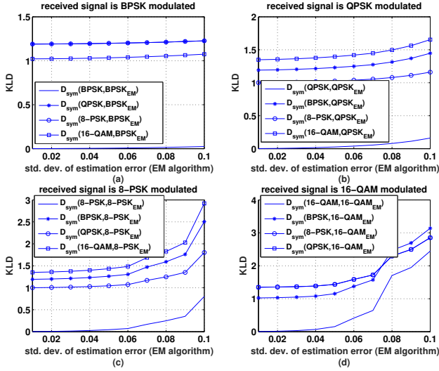
Fig. 9. Self-KLD and corresponding pair-wise symmetric KLDs for each of the four considered modulation schemes plotted against the (standard deviation of) estimation error of the EM algorithm. For this plot, number of Monte-Carlo simulations done was 1e4 . Furthermore, we set \sigma = 0.1 . For illustration, D_{sym}(QPSK, BPSK_{EM}) implies the pair-wise symmetric KLD between the Gaussian approximated pdf of the GMM of the template signal in the database representing QPSK modulation, and the Gaussian approximated pdf of the GMM of the received deconvolved signal containing BPSK modulation. Furthermore, the GMM parameters of the template signal are perfectly known, while the GMM parameters of the received deconvolved signal are learned via the EM algorithm.
