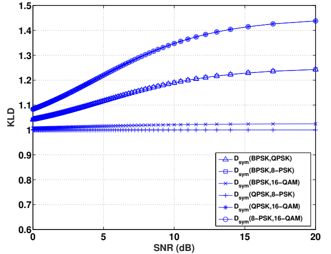
Fig. 8. Pair-wise symmetric KLDs for the considered modulation schemes against SNR. Note that the curve D_{sym}(\text{QPSK},16\text{-QAM}) is superimposed on D_{sym}(\text{8-PSK},16\text{-QAM}) , and the curve D_{sym}(\text{BPSK},\text{QPSK}) is superimposed on D_{sym}(\text{BPSK},8\text{-PSK}) .
