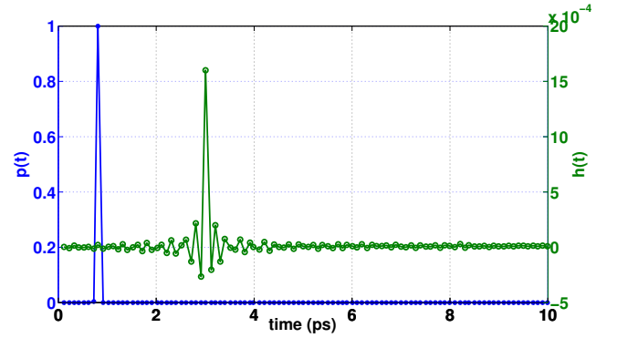
Fig. 2. THz channel impulse response h(t) observed at the nano receiver when a 100 femto seconds long Gaussian pulse p(t) is transmitted by the nano transmitter at t = 800 fs. Additionally, to obtain this plot, the nano receiver was placed at a distance of 1 mm from the nano transmitter [8].
