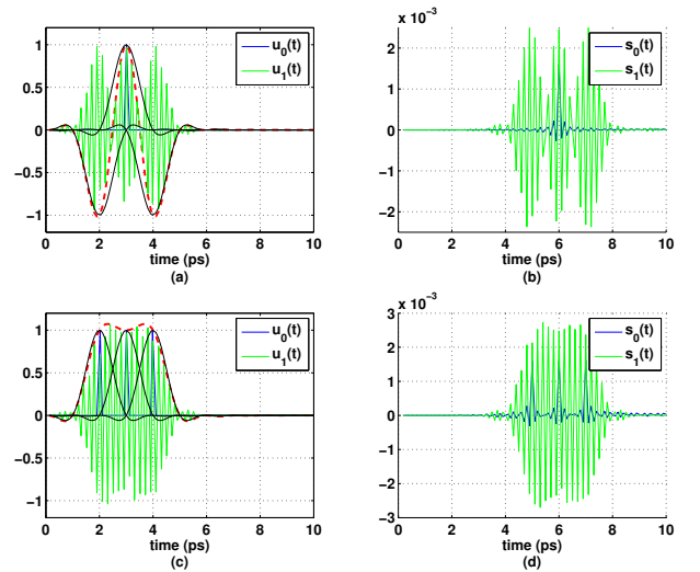
Fig. 3. Simulation setup for Mode detection: PBM approach utilizes OOK, while CBM approach utilizes BPSK scheme. For CBM approach, a carrier of frequency 5 THz was used. In Figs. 3(a)-(b), the transmitted symbol sequence is \{-1, +1, -1\} , while in Figs. 3(c)-(d), the transmitted symbol sequence is \{+1, +1, +1\} . Furthermore, in Figs. 3(a), (c), the red curve represents the envelope e_{u_1} = \sum_k b[k]q(t - kT) of u_1(t) , while each of the black curve represents q_k(t) = q(t - kT) for k \in \{2, 3, 4\} . Finally, the duty cycle of the Gaussian pulses is set to 10% under PBM approach.
