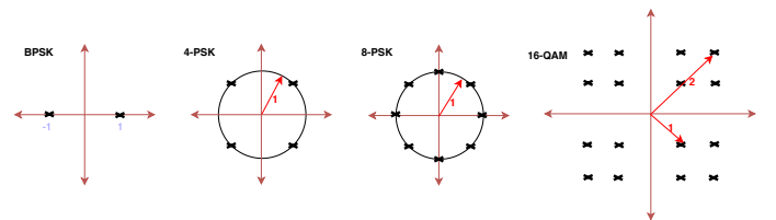
Fig. 6. Labelled constellation plots for the modulation schemes considered in this work.
