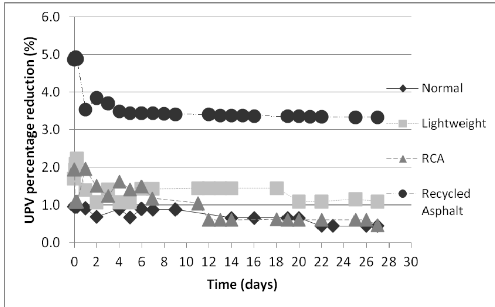
Fig. 7. Percentage reduction in UPV for concretes with normal, lightweight, RCA, and recycled asphalt aggregates.
