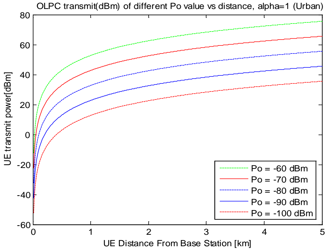
Figure 5.19 Required UE transmit with different base station sensitivity ( P_o ) with \alpha = 1 using the Okumura-Hata urban model
