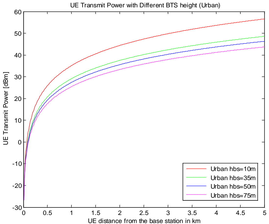
Figure 5.6 Required UE transmit power from the base station with different height of base station for urban
