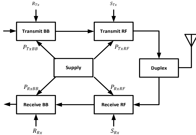
Figure 3.1 LTE UE physical layer
