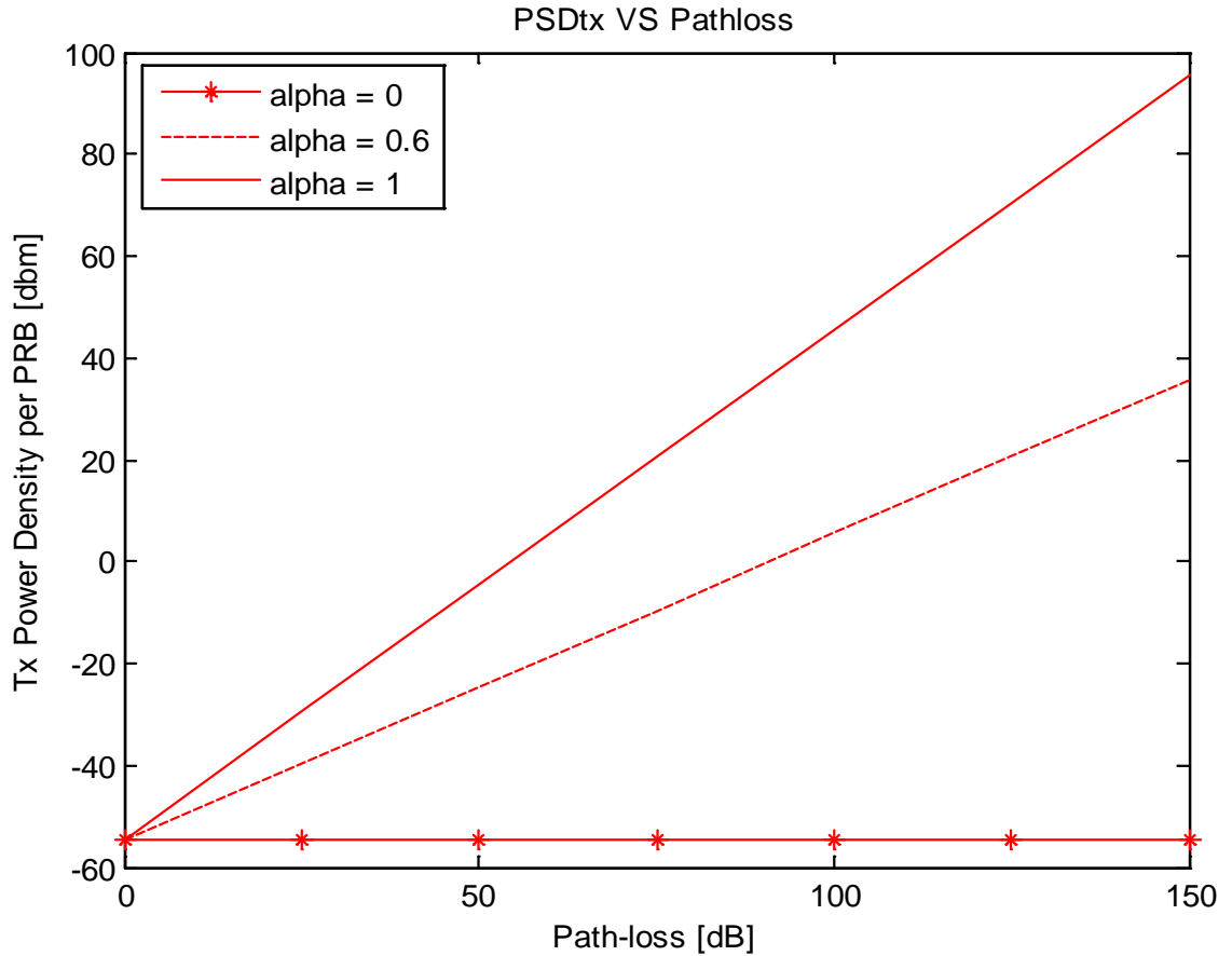
Figure 5.9 PSD_{tx} Vs Path-loss ( P_L ) for \alpha = 0, 0.6 and \alpha = 1
