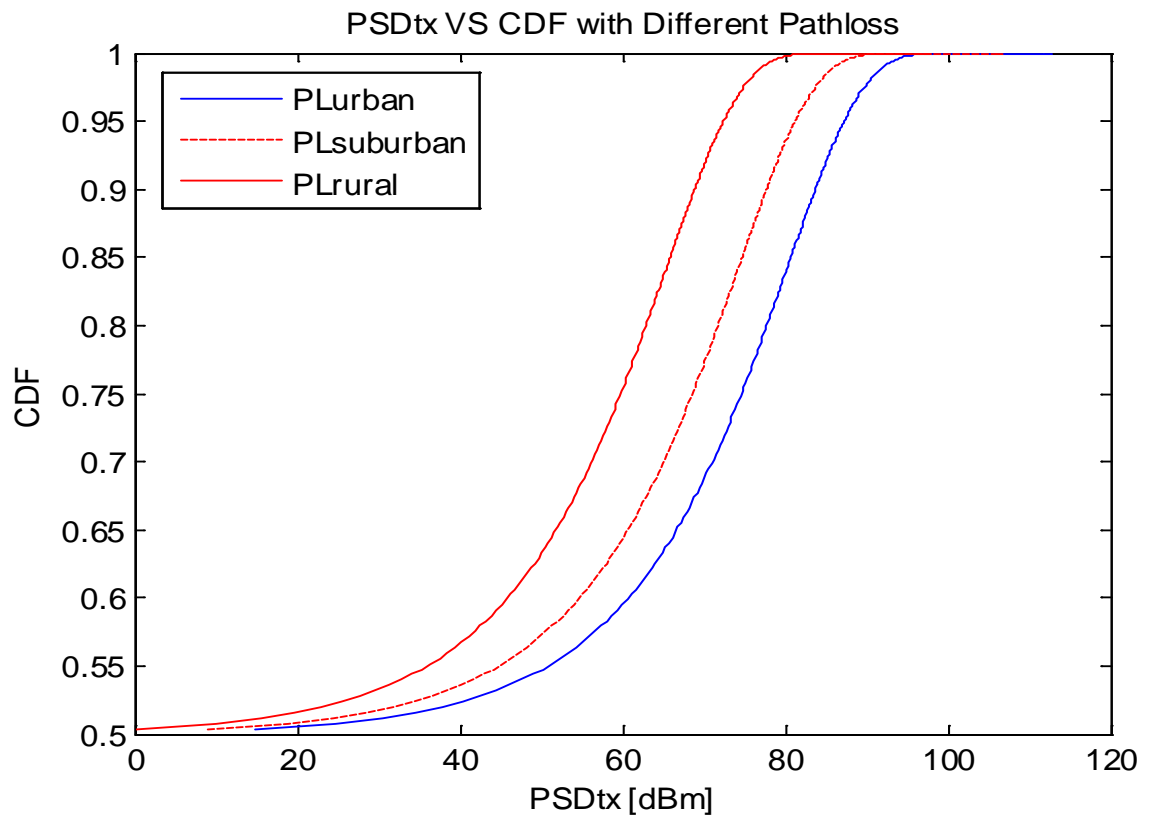
Figure 5.2 Required UE transmit power with different path losses
