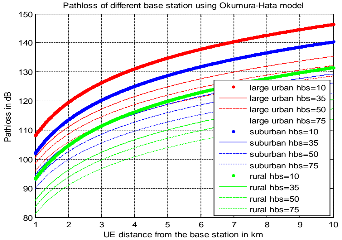
Figure 5.1 Okumura-Hata Propagation model path loss
