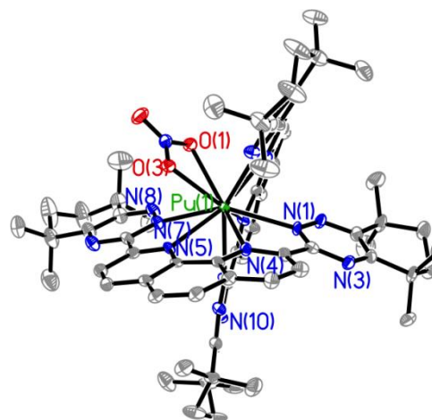
Figure 2. Thermal ellipsoid plot of the solid-state structure of [\text{Pu}^{\text{III}}(\text{CyMe}_4\text{-BTPPhen})_2(\text{NO}_3)]_2[\text{Pu}^{\text{IV}}(\text{NO}_3)_6] \cdot 4\text{MeCN} . The [\text{Pu}^{\text{IV}}(\text{NO}_3)_6]^{2-} anion, lattice solvent, and H atoms have been omitted for clarity.
