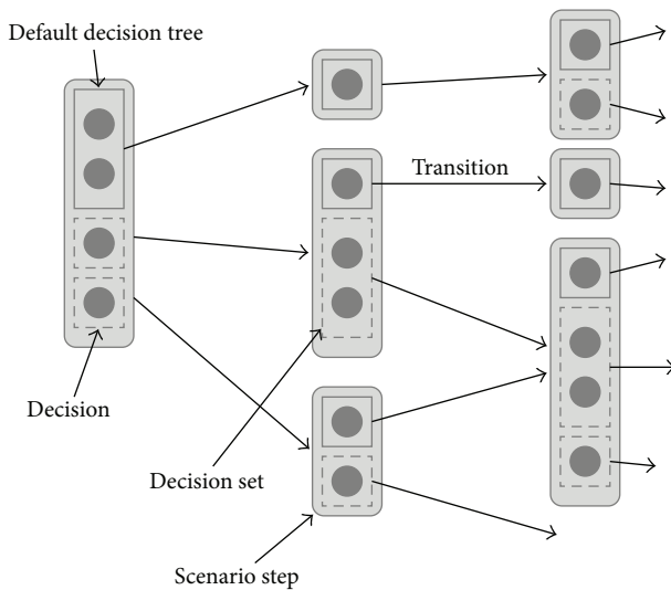
FIGURE 11: Decision tree.
