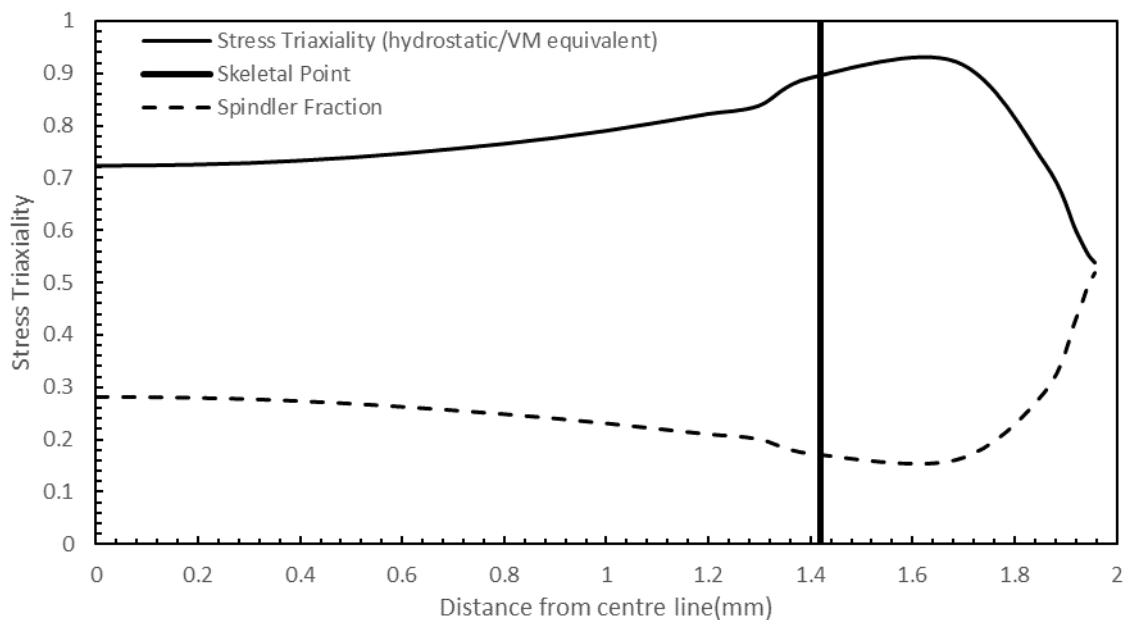
Figure 7 – Stress triaxiality and Spindler Fraction along the centre line after loading up to 342MPa (no creep)
