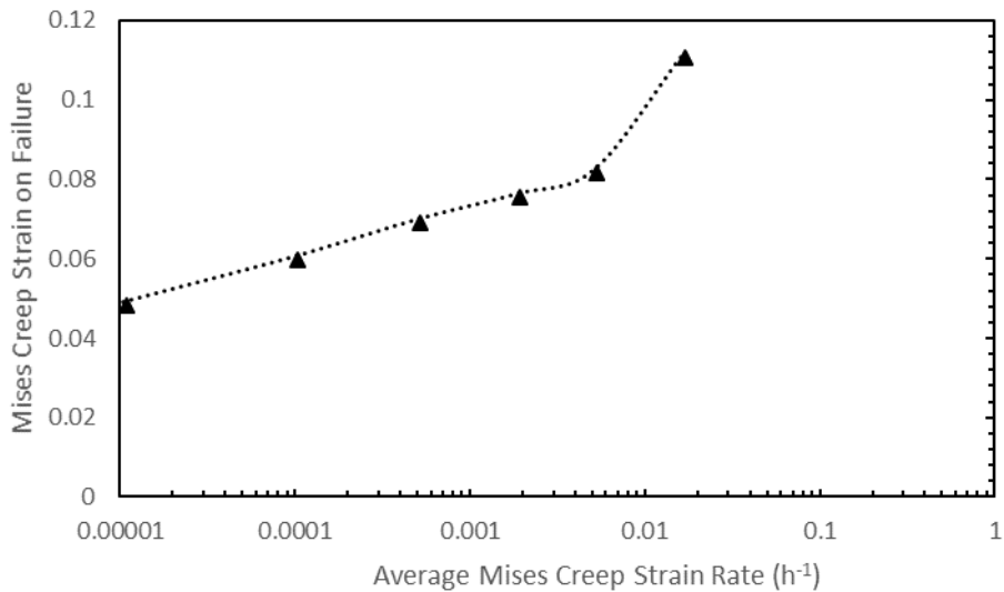
Figure 9- Mises creep strain on failure against average Mises creep strain rate (FEA) at the point of maximum damage
