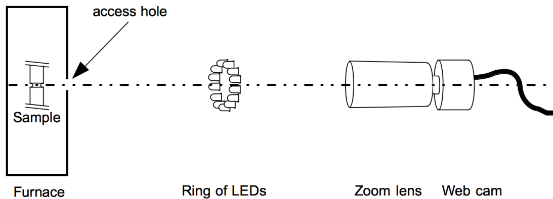
Figure 1 - Camera set up for notch imaging
