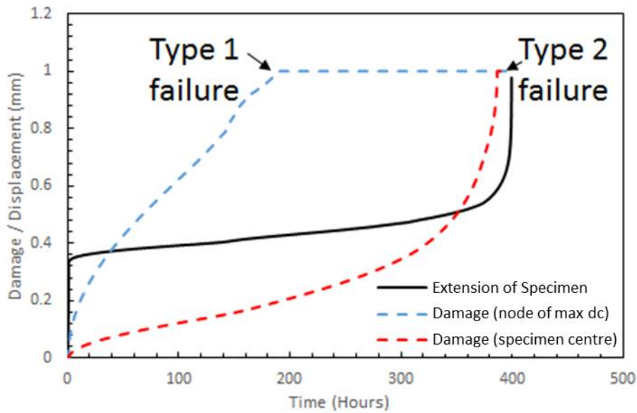
Figure 10 - Creep damage accumulation over time leading to failures (Net section stress 390MPa (FEA extension shown))
