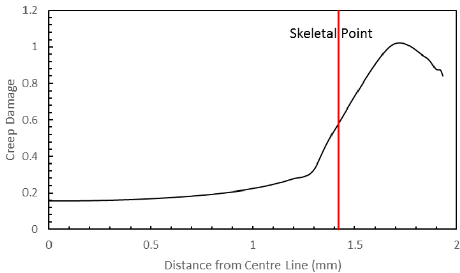
Figure 11 - Creep damage predicted across ligament as first element fails (Type 1 failure distribution)
