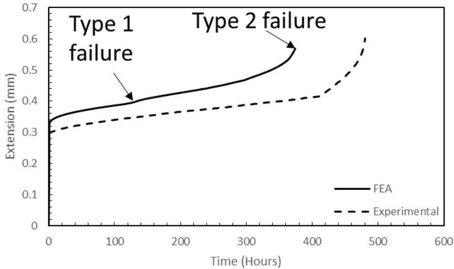
Figure 8 - Notched bar with applied net section stress 390MPa
