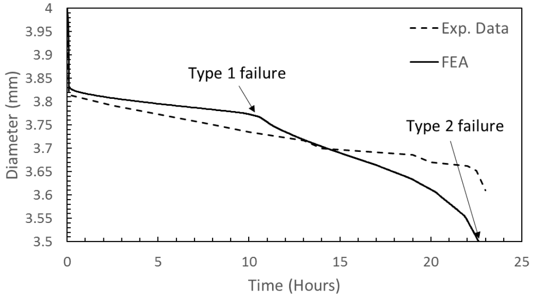
Figure 12 - Reduction in diameter, 500MPa net section stress (data from camera)
