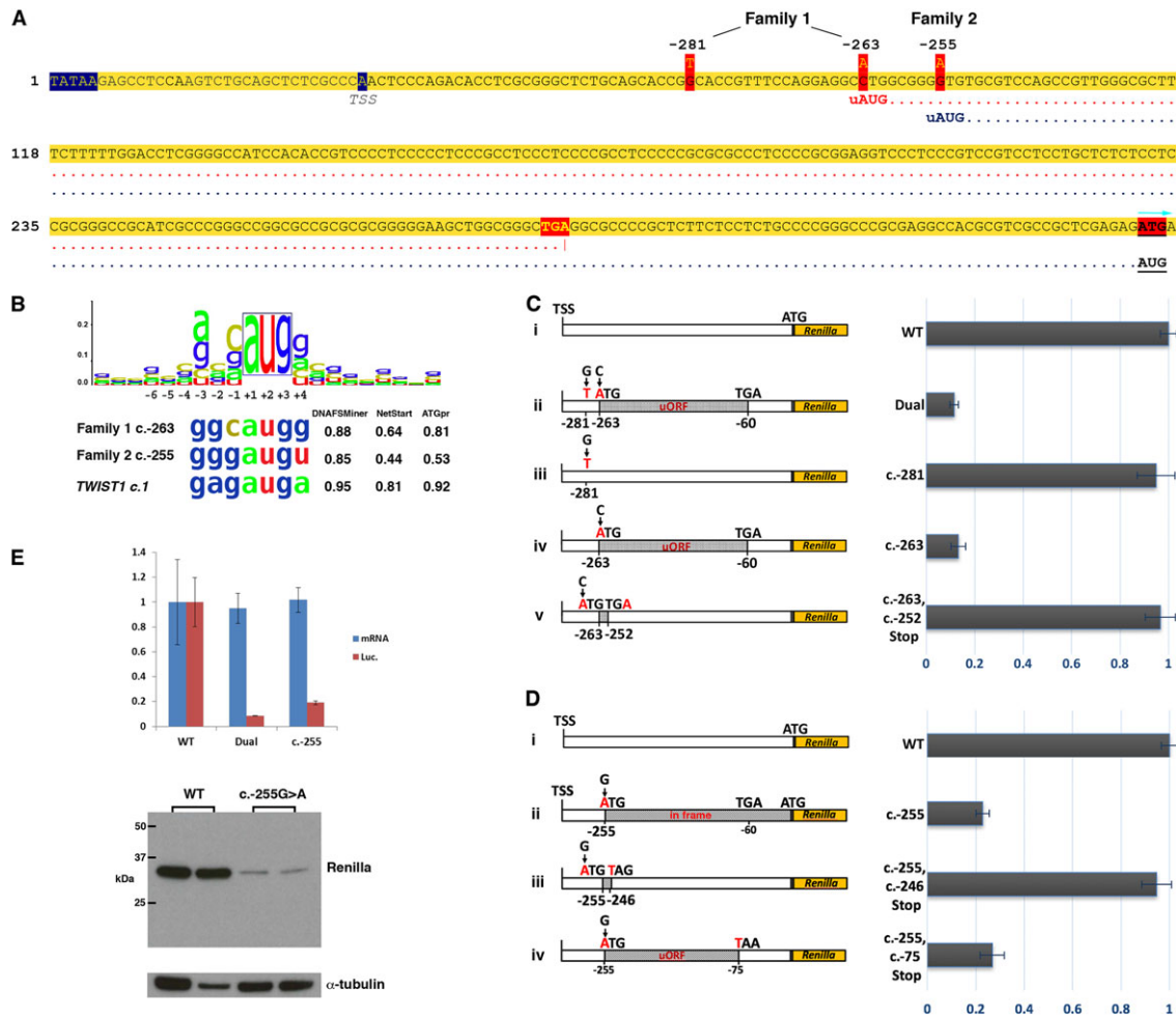
FIGURE 2 Twist1 5' UTR variants and effect on translation. A: Genomic sequence showing the locations of the variants identified in Families 1 and 2 within the 5' UTR of Twist1 (NM_000474.3). The TATAA box and transcription start site (TSS) are denoted by blue shading. The reading frames from the uAUGs at -263 (Family 1) and -255 (Family 2) are indicated by red and blue dotted lines, respectively. Note that the ORF from c.-263 terminates at a stop codon (TGA; yellow text with red shading) that is 62 bp upstream of the reference start codon of Twist1 (denoted by red highlighting and turquoise arrow). The uAUG in Family 2 is in-frame with the Twist1 start codon. B: Kozak consensus sequence (Kozak, 1986) aligned to the uAUGs of Families 1 and 2, and to the Twist1 start codon (sAUG). The relative strengths of these possible translation initiation sequences were assessed by three online tools, DNA functional site miner (DNAFSMiner), NetStart, and ATGpr with scores shown on the right. C: Luciferase analysis to determine the effect of the Family 1, 5' UTR variants on translation. Luciferase reporter DNA constructs are shown on the left and normalized luciferase activity generated from each is shown on the right. (i) WT construct. (ii) The Dual construct contains both c.-263 and c.-281 variants, while the c.-281 (iii) and c.-263 (iv) constructs contain each variant in isolation. The c.-263C > A variant is in-frame with a TGA stop codon at c.-62_60 generating a large uORF of 204 bp (grey shading; 68 codons). (v) The c.-263, c.-252Stop construct incorporates a new stop codon at -254_252, shortening the uORF to four codons and extending the distance from the uORF to the mORF from 59 bp to 251 bp. D: Luciferase analysis of the Family 2 variant c.-255G > A. (i) WT construct. (ii) The ATG created by c.-255 is in-frame with the luciferase ORF adding a further 85 codons. (iii) The c.-255, c.-246Stop construct incorporates a new stop codon at -246_244 to create a short four codon uORF, while the c-255, c-75Stop construct (iv) contains a longer uORF of 61 codons. Plots are shown as mean \pm standard error based on three separate experiments carried out in triplicate. E: The top panel shows RT-qPCR (blue) and dual luciferase reporter (red) assays in HEK 293T cells comparing Renilla luciferase expression and activity using WT, Dual, and c.-255 constructs (plots are shown as mean \pm SD). The y-axis shows relative expression or activity of the Renilla reporter gene (normalized against firefly and to WT). mRNA levels and luciferase activity are indicated in blue and red, respectively. Bottom panel: western blot analysis of transfected HEK293 cell lysates showing expression of Renilla luciferase produced from WT (lanes 1 and 2) and c.-255 constructs (lanes 3 and 4), from separate experiments. The N-terminal extension produced by translation from c.-255 uAUG is predicted to increase the molecular weight of Renilla by ~9 kDa, but a larger product was not detected. Anti- Renilla luciferase antibody (Abcam ab185925) and \alpha -tubulin (Santa Cruz, sc-32293) at 1/1000 dilutions were used against 10 \mu g of protein lysate (BCA protein assay kit, Thermo)
