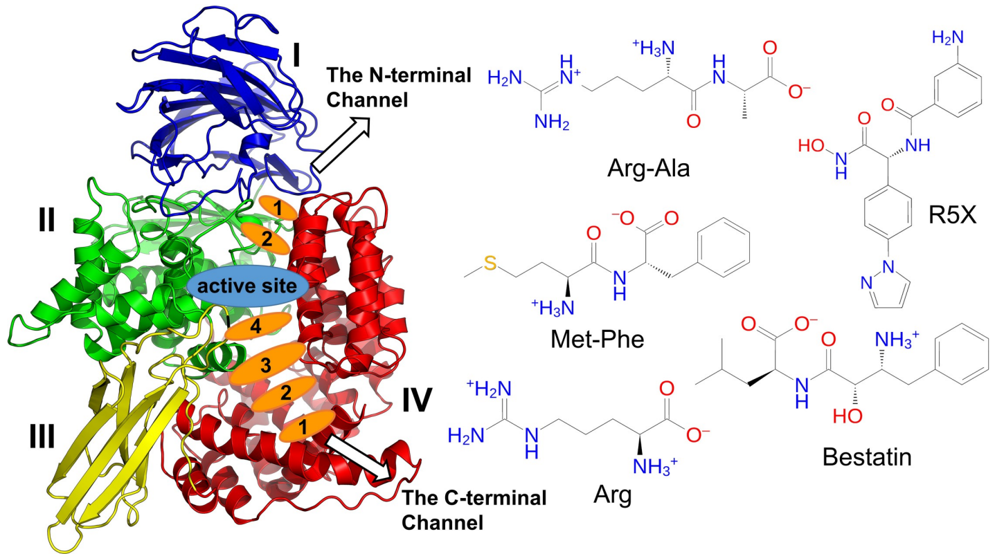
Fig 1. The Plasmodium falciparum M1 alanyl aminopeptidase ( PfM1 -AAP) with the substrates (Arg-Ala and Met-Phe), inhibitors (Bestatin and R5X) and Arg product. The PfM1 -AAP domains are coloured and labelled. The long C-terminal and short N-terminal channels and the position of residues selected for calculation of R_{\text{gr}} are shown.
