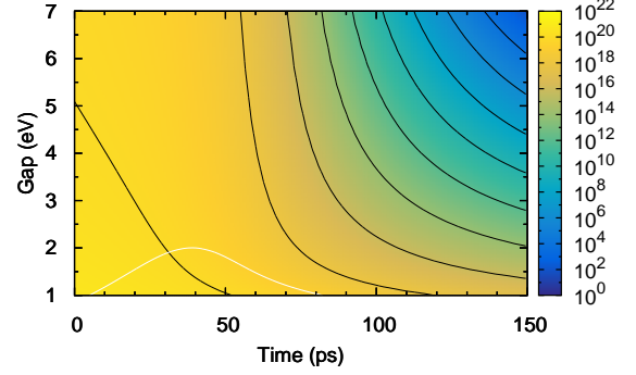
Figure 2. Map of the electron-hole pair density as function of the band gap and time, at fixed molar density. The the band gap of BK7 glass is approximately 3.5 eV, see text for the fixed model parameters. In the the region below the white line the electron-hole plasma is degenerate.
