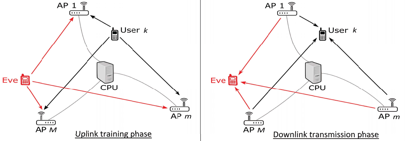
Fig. 1. A system model consisting of M APs, K legal users and one active eavesdropper Eve. The arrows point to the direction from transmitters to receivers. All directions, connected to Eve, are in red. In uplink training phase, all users and Eve send the pilots to the APs in order to request for the messages, which privately intended for them. Connected together through a CPU, the APs exchange information, estimate channels and detect abnormality in pilot sequences. In downlink transmission phase, the APs transmit their designed signals to users and Eve.
