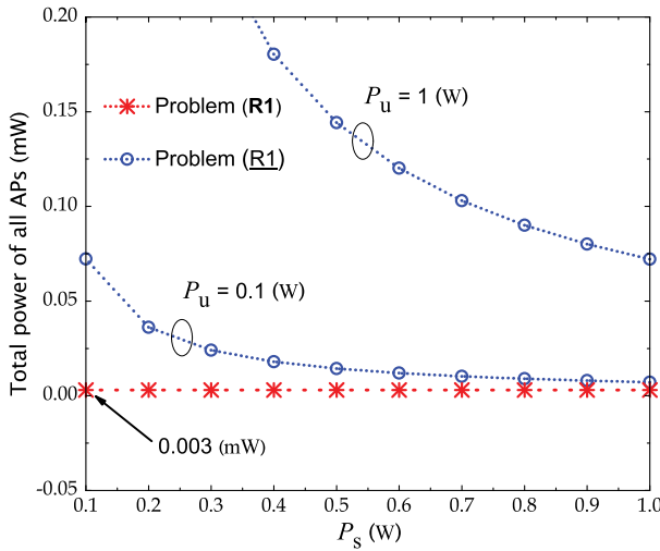
Fig. 6. Total power of all APs (in mW) versus P_s (the average transmit power for a signal s_k ). Other parameters: the average transmit power of each user is P_u = \{0.1, 1\} W, the average transmit power of Eve is P_E = 0.5 W, M = 50 , K = 8 , T = 12 , \theta_1 = 0.1 , \theta_k = 0.02 for k = \{2, \dots, K\} and \theta_E = \theta_1/50 .
