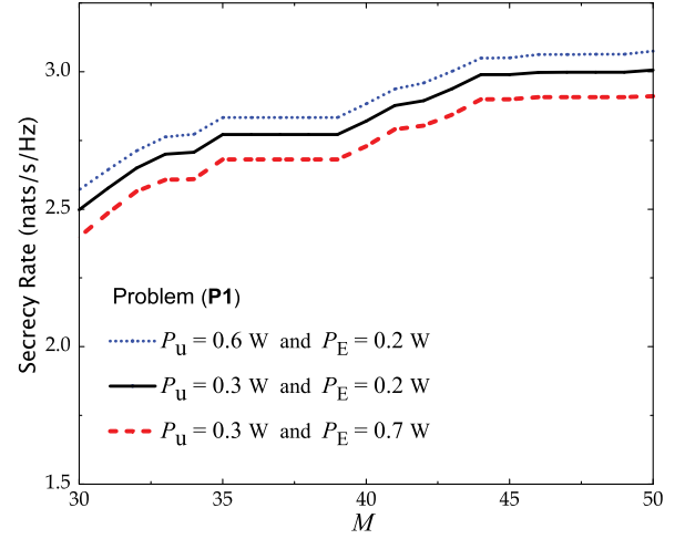
Fig. 4. Secrecy rate versus M . Other parameters: the average transmit power for a signal s_k is P_s = 0.8 W, the average transmit power of each user is P_u = \{0.3, 0.6\} W, the average transmit power of Eve is P_E = \{0.2, 0.7\} W, K = 8 , T = 12 , \theta_k = 2 \times 10^{-4} for k = \{2, \dots, K\} and \theta_E = \theta_k/50 .
