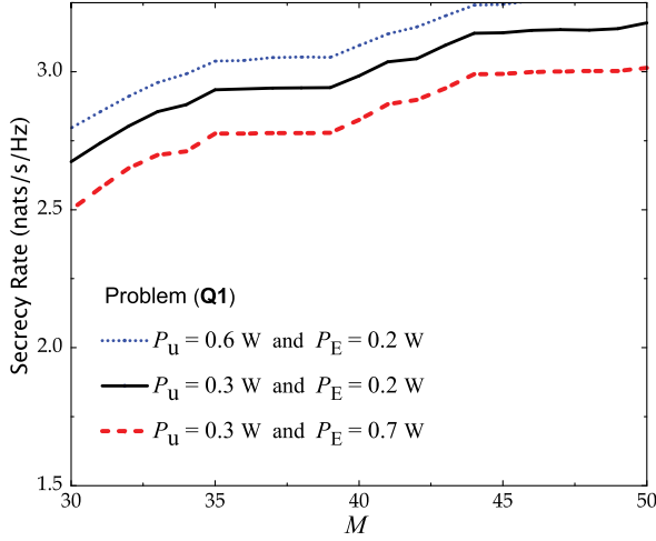
Fig. 5. Secrecy rate versus M . Other parameters: the average transmit power for a signal s_k is P_s = 0.8 W, the average transmit power of each user is P_u = \{0.3, 0.6\} W, the average transmit power of Eve is P_E = \{0.2, 0.7\} W, K = 8 , T = 12 and \theta_k = 2 \times 10^{-4} for k = \{2, \dots, K\} .
