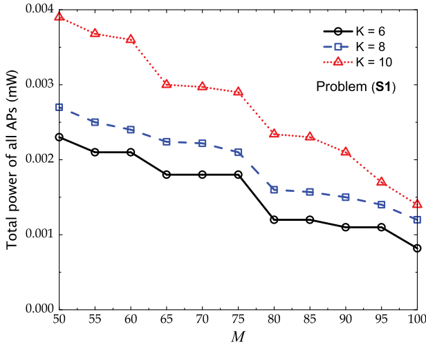
Fig. 9. Total power of all APs (in mW) versus M . Other parameters: the average transmit power for a signal s_k is P_s = 0.7 W, the average transmit power of each user is P_u = 0.4 W, the average transmit power of Eve is P_E = 0.5 W, K = \{6, 8, 10\} , T = 12 , \theta_k = 0.02 for k = \{2, \dots, K\} and \phi = 1 .
