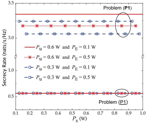
Fig. 2. Secrecy rate versus P_s (the average transmit power for a signal s_k ). Other parameters: the average transmit power of each user is P_u = \{0.3, 0.6\} W, the average transmit power of Eve is P_E = \{0.1, 0.5\} W, M = 50 , K = 8 , T = 12 , \theta_E = 10^{-4} , and \theta_k = 2 \times 10^{-4} for k = \{2, \dots, K\} .
