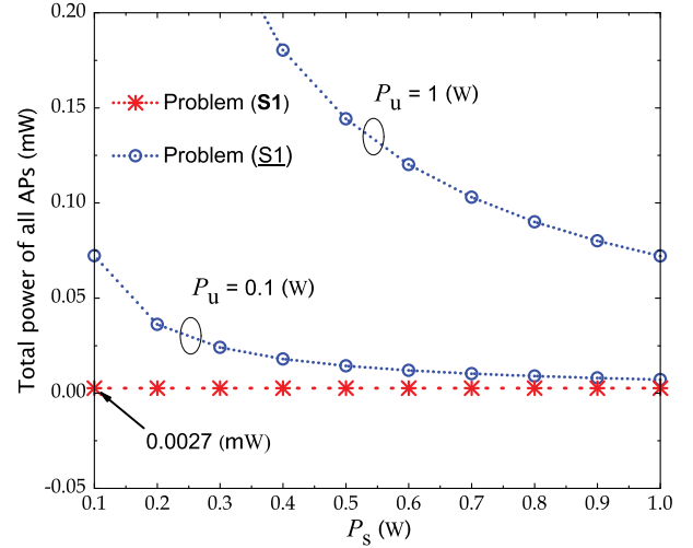
Fig. 7. Total power of all APs (in mW) versus P_s (the average transmit power for a signal s_k ). Other parameters: the average transmit power of each user is P_u = \{0.1, 1\} W, the average transmit power of Eve is P_E = 0.5 W, M = 50 , K = 8 , T = 12 , \theta_k = 0.02 for k = \{2, \dots, K\} and \phi = 1 .
