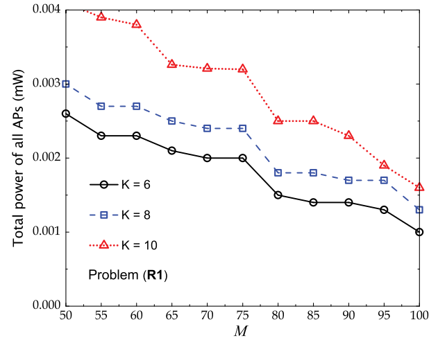
Fig. 8. Total power of all APs (in mW) versus M . Other parameters: the average transmit power for a signal s_k is P_s = 0.7 W, the average transmit power of each user is P_u = 0.4 W, the average transmit power of Eve is P_E = 0.5 W, K = \{6, 8, 10\} , T = 12 , \theta_1 = 0.1 , \theta_k = 0.02 for k = \{2, \dots, K\} and \theta_E = \theta_1/50 .
