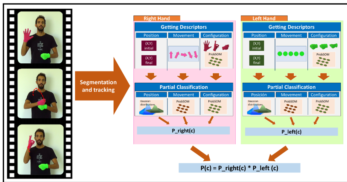
Figure 1. Classification model
