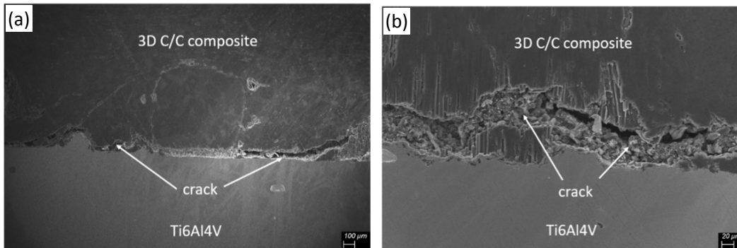
Fig. 5. The interface of the joints between the flat surface 3D C/C composite and Ti6Al4V with two different imaging resolutions.
