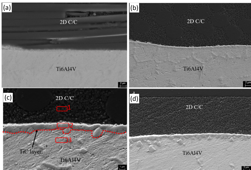
Fig. 3. (a) the interface between the 2D C/C composite and Ti6Al4V for a welding current of 4 kA, (b) 5 kA, (c) 6 kA and (d) 8 kA. EDS analysis was performed on areas of 1, 2 and 3 in (c), as described in the text.
