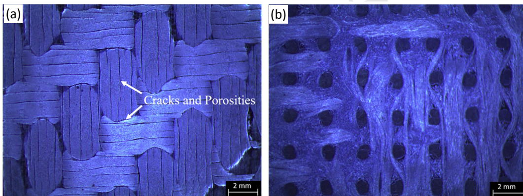
Fig. 2. Optical images of the surface of (a) the 2D C/C composite and (b) the 3D C/C composite.
