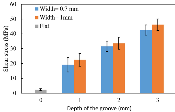
Fig. 12. Shear strength of the 3D C/C composite-Ti6Al4V joints for flat and groove-patterned interfaces with a groove depth between 1 to 3 mm and a width between 0.7 to 1 mm.
