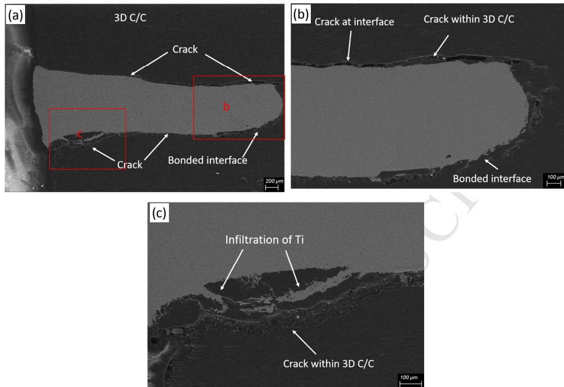
Fig. 15. Cross sections of the microstructure's fractured Ti indentation for the 3D C/C composite-Ti6Al4V joint after a shear test for a groove depth of 3 mm.
