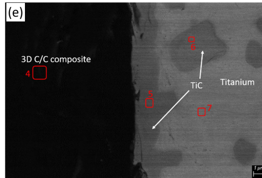
Fig. 7. SEM images of the cross section of the joint between the 3D C/C composite and Ti6Al4V with the groove width of 1 mm and depth of 3 mm: (a) the panorama of the joint interface, where (b), (c), (d) and (e) are zoomed-in images of the selected area in (a).
