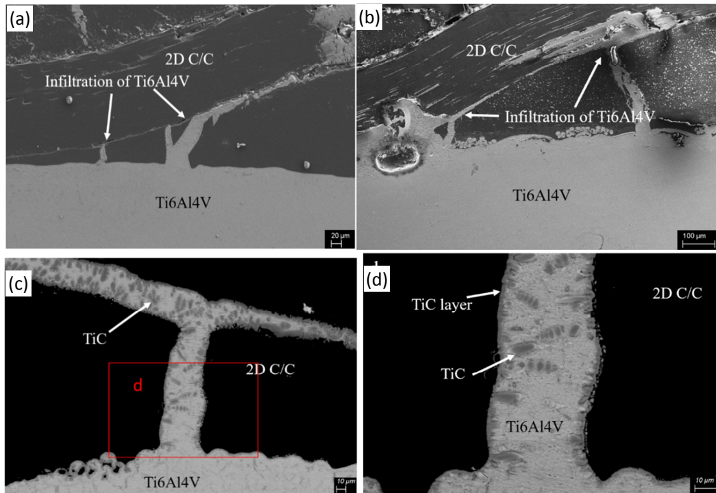
Fig. 4. Typical images showing the penetration and infiltration of the melted Ti6Al4V into the pores and cracks of the 2D C/C composite for a welding current of (a) 5 kA and (b) 6 kA. (c): SEM-backscattered image for 6 kA and (d): zoom-in image of the selected area in (c).
