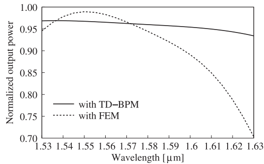
(a) output power spectrum in port 2
