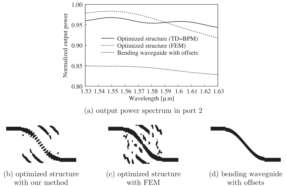
Fig. 3. Optimization results of bending waveguide.
