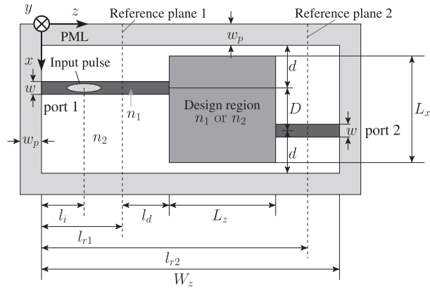
Fig. 1. Design model for bending waveguide.
