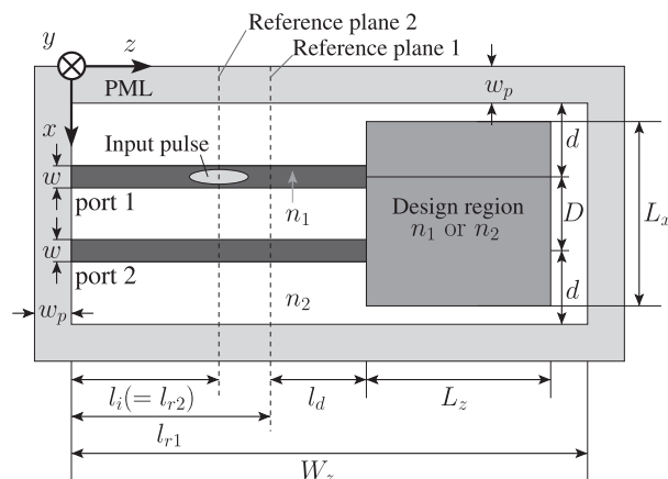
Fig. 4. Design model for reflector.
