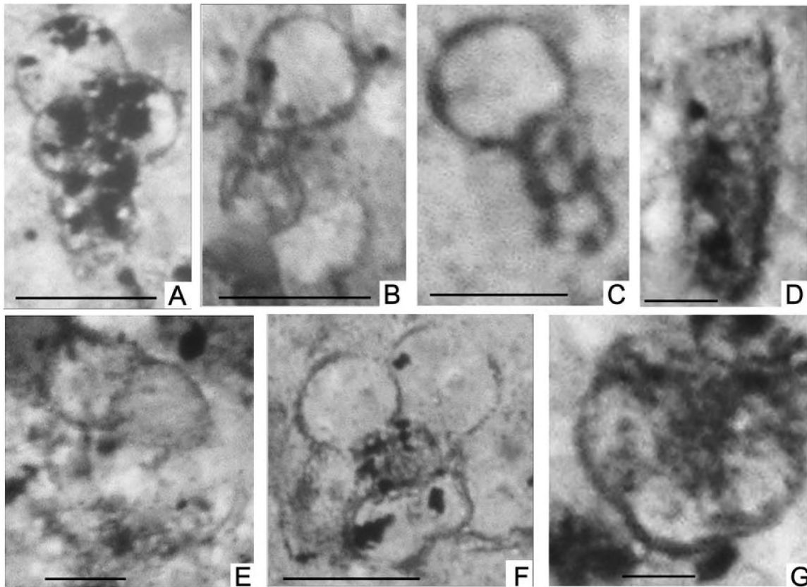
Fig. 7. Redeposited planktonic foraminifera from the uppermost part of the Middle Lgota Beds
