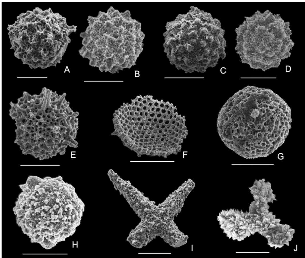
Fig. 6. Spumellaria from the Mikuszowice Cherts
