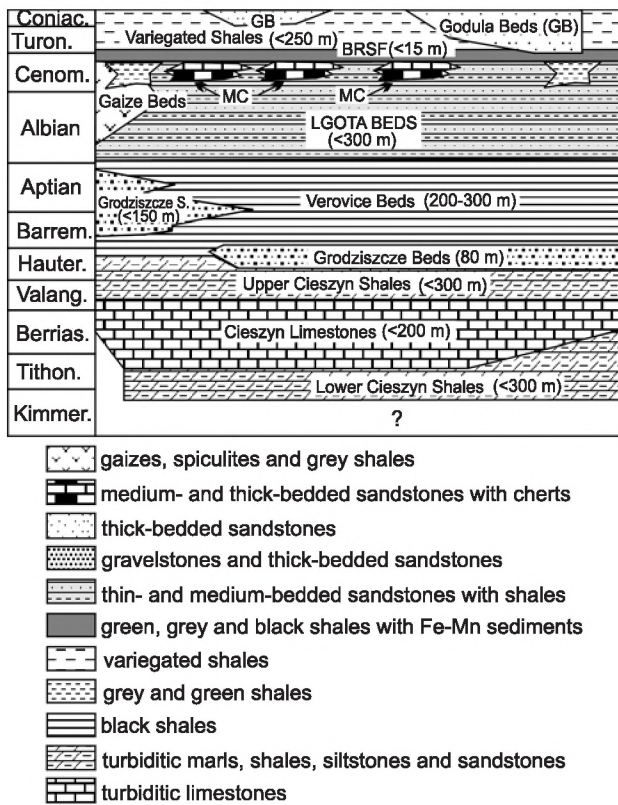
Fig. 2. Generalized stratigraphy of the Kimmeridgian-Coniacian of the Silesian Nappe after Koszarski and Słaczka (1973), slightly modified
