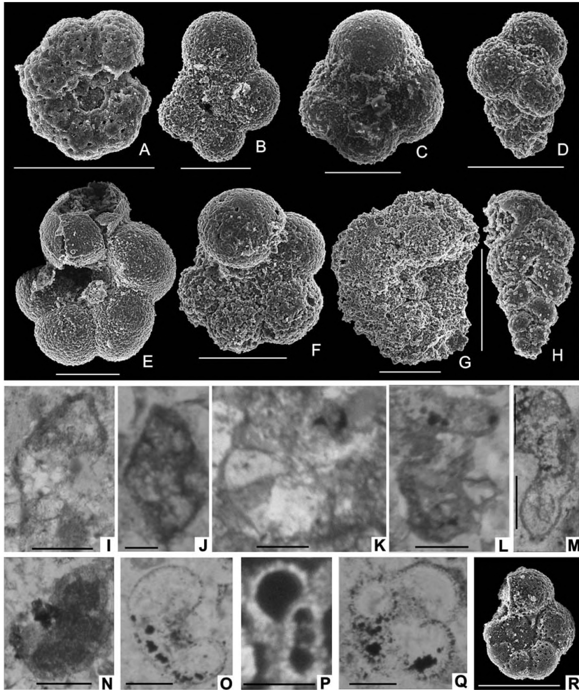
Fig. 8. Redeposited planktonic foraminifera from the Mikuszowice Cherts
