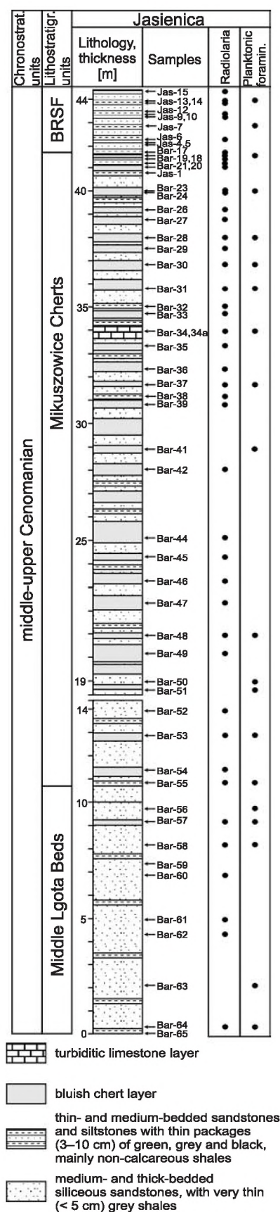
Fig. 3. Stratigraphic log of the Mikuszowice Cherts and the encompassing units at the Jasienica section, with positions of the samples studied and occurrences of radiolaria and planktonic foraminifera
