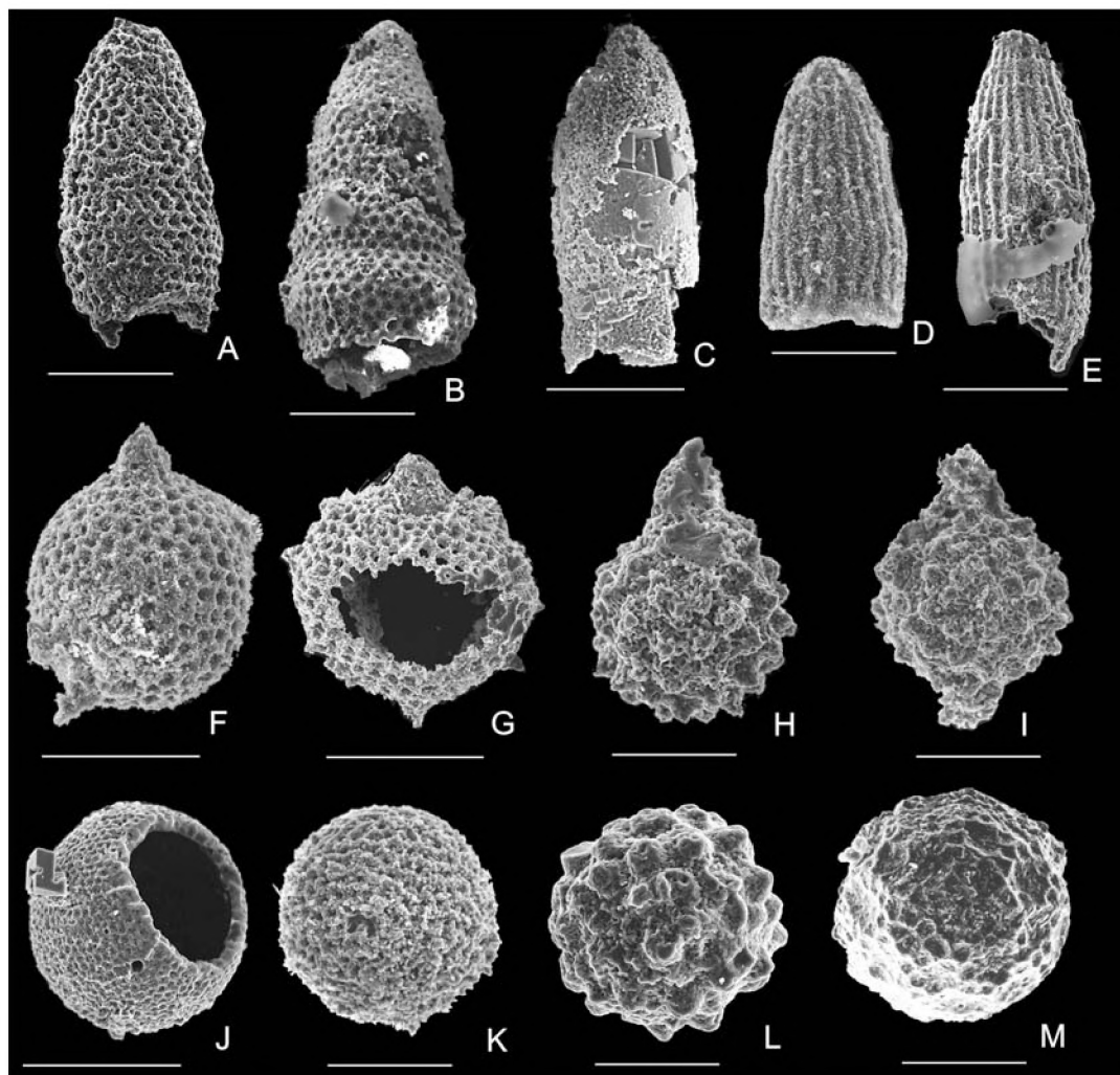
Fig. 5. Nassellaria from the Mikuszowice Cherts and surrounding units
