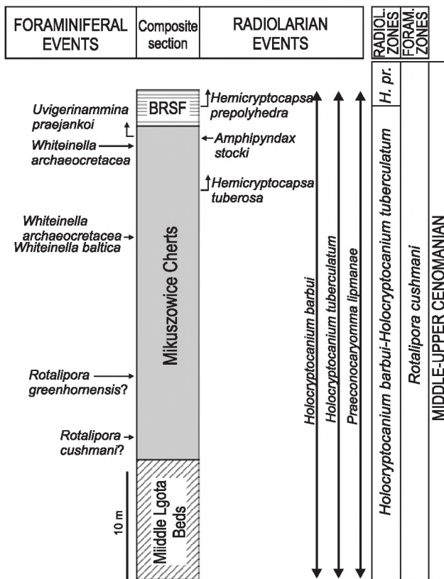
Fig. 9. Composite section of the Mikuszowice Cherts and the encompassing adjoining units at the Barnasiówka Range (Silesian Nappe, Outer Carpathians) with the stratigraphically important radiolarian and foraminiferal datum events. Note that the planktonic foraminiferal zone is here approximately indicated based on comparisons of radiolarian ranges from pelagic, calcareous facies
