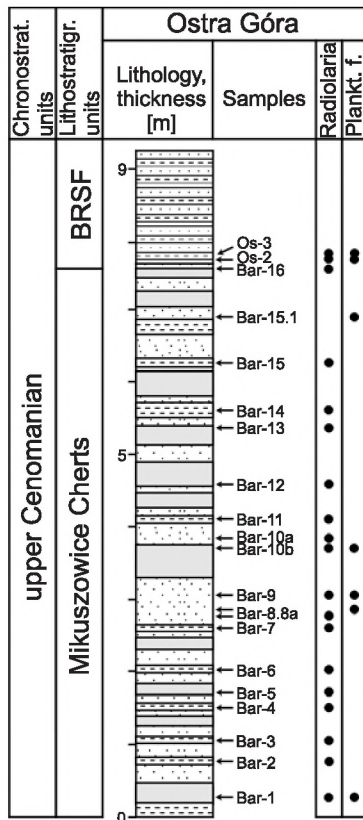
Fig. 4. Stratigraphic log of the upper part of the Mikuszowice Cherts and the lowermost part of the Barnasiówka Radiolarian Shale Formation (BRSF) at the Ostra Góra section with positions of the samples studied and occurrences of radiolaria and planktonic foraminifera
