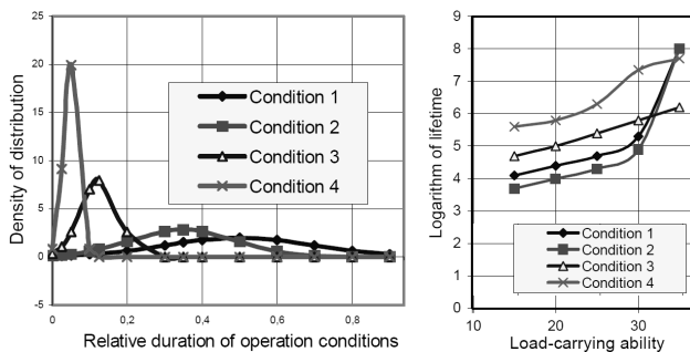
Fig. 9 – Representation of operation conditions (left) and lifetime-strength curves of a component (right)
