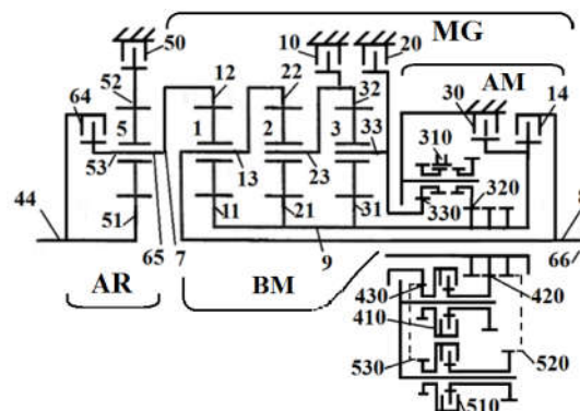
Fig. 3 – One of the synthesized transmission
