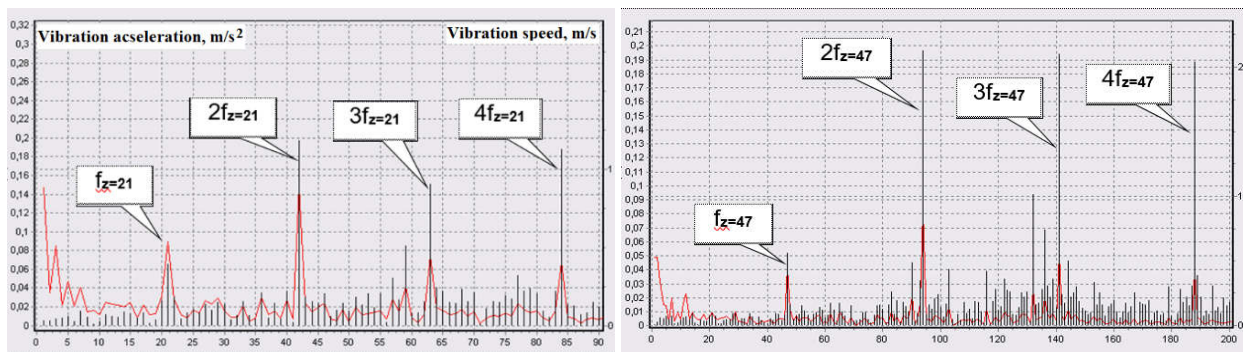
Fig. 13 – Harmonic spectra of vibrations generated by the sun gear (left, 21 teeth) and satellites (right, 47 teeth) of the RMW planetary row
