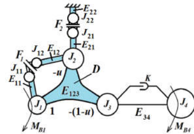
Fig. 8 – Stiff-elastic (left) and normalized (right) diagrams
