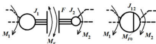
Fig. 6 – States of a friction clutch: slipping (left) and locking (right)
