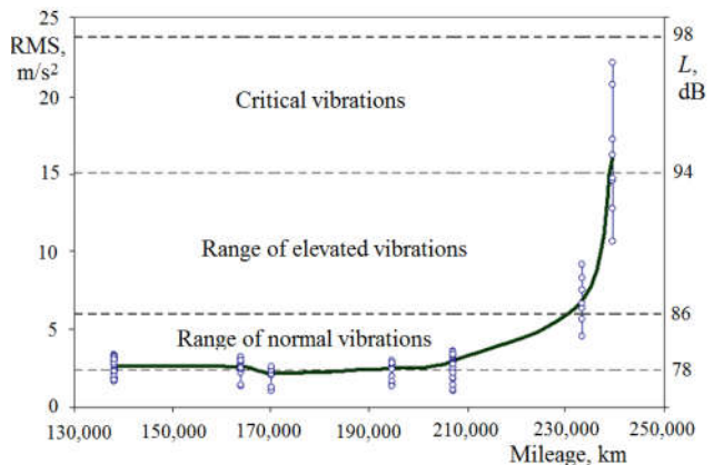
Fig. 14 – Dependence of RMS values of vibration acceleration of RMW on the mileage of a dump truck
