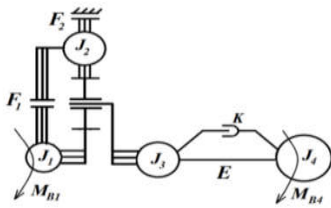
Fig. 7 – Stiff-elastic RMS
