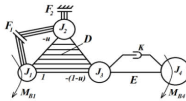
Fig. 8 – Stiff-elastic (left) and normalized (right) diagrams
