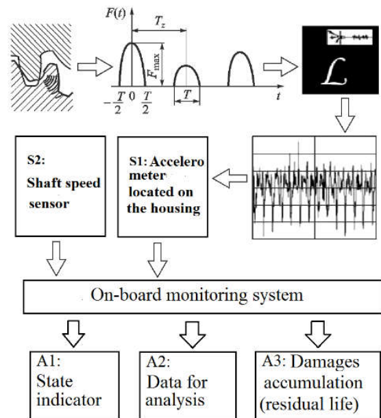
Fig. 12 – Processes in the RMW monitoring system
