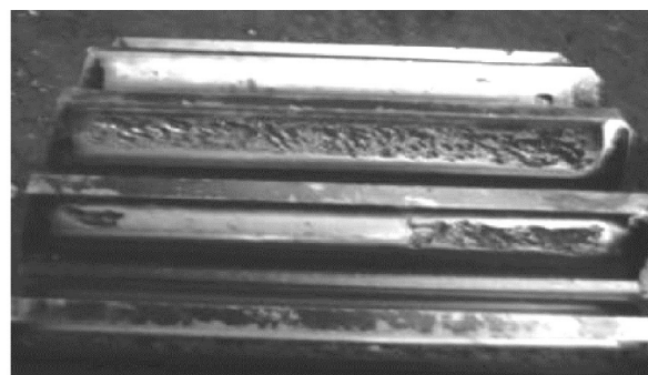
Fig. 15 – Damaged working surfaces of the sun gear teeth
