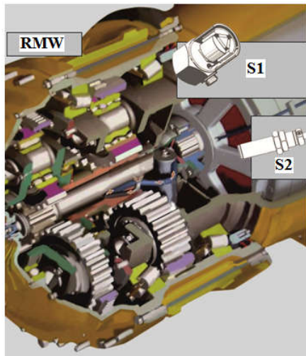
Fig. 11 – RMW with sensors
