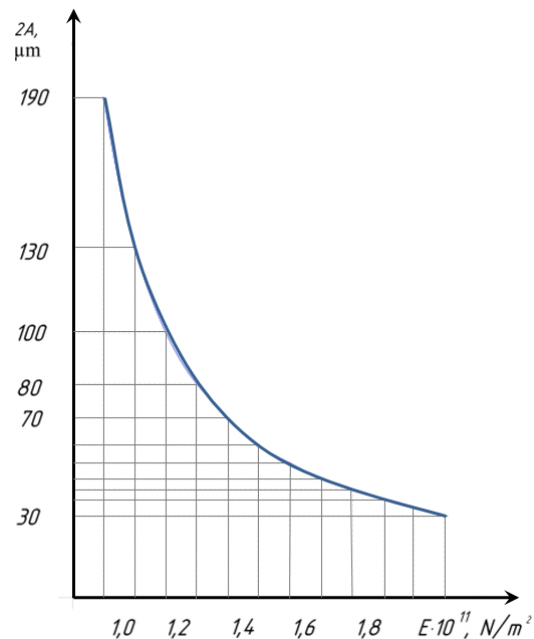
Fig. 7 – Dependence of double amplitude of vibration from the elasticity modulus of the core
