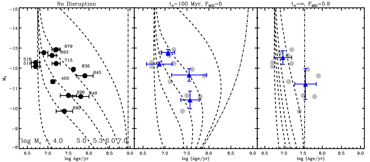
Fig. 2. Age vs. M_V for the twelve clusters in the present study. In each panel, we also show the expectations of the median M_V for a given age, following the results of Larsen (2009). The model disruption parameters are given at the top of each panel, where \hat{t}_4 is the disruption timescale of a 10^4 M_\odot cluster in the mass dependent cluster disruption scenario, and F_{\text{MID}} is the fraction of clusters destroyed every decade in age. The dashed lines represent models with different values of the Schechter truncation mass, and the dashed-dot lines in each panel represents the case without truncation (i.e., a pure power-law). In the middle and right panels, the original data are shown in grey, while the binned data (the mean in flux and age, with the error bars representing the standard deviation) are shown as solid (blue) triangles. Two different bin sizes are shown.
