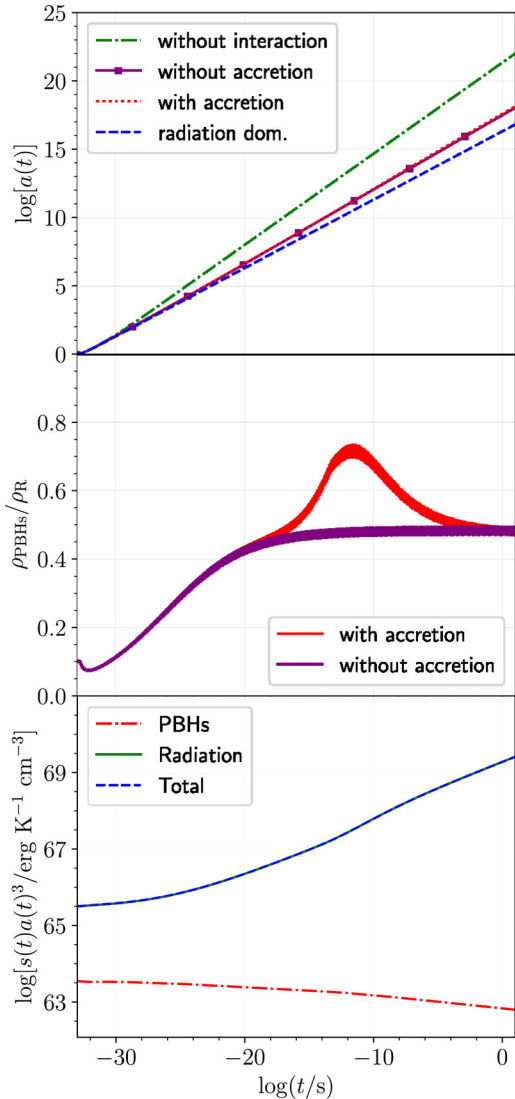
Figure 5. Cosmic evolution for a power-law IMF with spectral index \gamma = 2.1 , and with masses lying between M_{\min} = 650m_{\text{p}} and M_{\max} = 10^6 M_{\odot} , for a value of \beta = 10^{-1} . Top panel shows the scale-factor evolution in four cases: with and without accretion, in a radiation-dominated universe, and in a universe with radiation and PBHs but without any interaction between them. Central panel shows the ratio of the fluid energy densities with and without accretion. Bottom panel shows the entropy per unit of comoving volume of both fluids as well as the total one.
