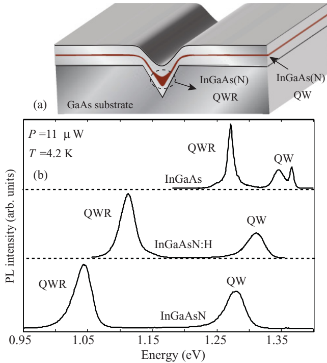
FIG. 1. (Color online) (a) Sketch of the QWR structure. (b) Micro-photoluminescence spectra ( T = 4.2 \text{ K} , P = 11 \mu\text{W} , B = 0 \text{ T} ) of the investigated QWR samples (from bottom to top: untreated InGaAsN, fully hydrogenated InGaAsN, and InGaAs).
