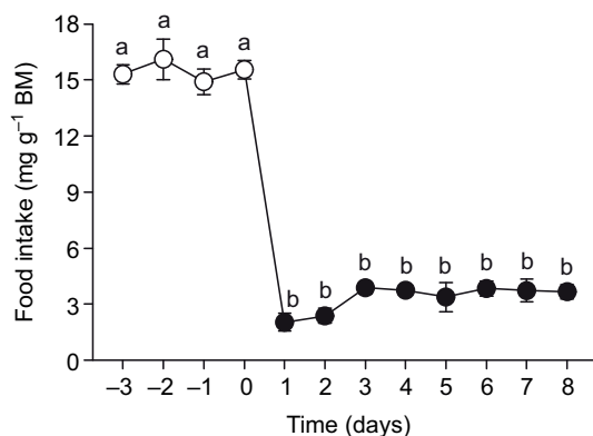
Fig. 1. Food intake in common carp exposed to normoxic (75% \text{O}_2 saturation; white circles) or hypoxic (10% \text{O}_2 saturation; black circles) water. The normoxic water source was replaced with a hypoxic source immediately after the assessment of food intake on day 0. Values that do not share a common letter are significantly different from each other as determined by repeated-measures one-way ANOVA and a Holm–Sidak multiple comparison test ( P < 0.05 ). Values are means \pm s.e.m. ( N = 3 tanks with nine fish per tank). BM, body mass.
