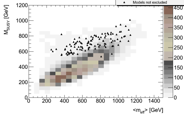
Figure 5. The distribution of m_{SUSY} to the average value of m_{eff} for excluded points (colour scale) and not excluded points (black dots).
