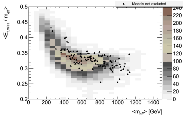
Figure 6. The distribution of the average value E_T^{miss}/m_{eff} to the average value of m_{eff} for excluded points (colour scale) and not excluded points (black dots).
