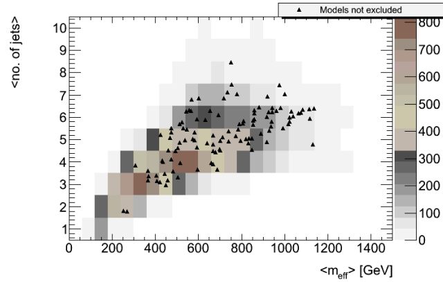
Figure 7. The distribution of the average value of m_{eff} to the average number of jets for excluded points (colour scale) and not excluded points (black dots).
