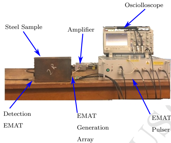
Figure 12: Schematic diagram of the experimental setup. The EMAT pulser (described in figure 2) drives the EMAT generation array (described in figure 11), which generates a focused longitudinal ultrasound wave. This is detected on the opposing side of the as-cast steel slab sample by the detection EMAT (described in figure 10). The signal is passed through an amplifier before being recorded on an oscilloscope.
