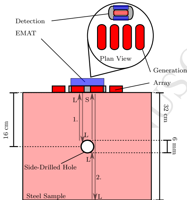
Figure 15: Schematic diagram of the pulse-echo experiment setup. The coil configuration shown was chosen to minimise exposure of the detection coil to magnetic flux from the generation coils and to minimise sensitivity to generated Rayleigh waves, which propagate perpendicular to the long axis of the coil. Path 1 corresponds to an incident longitudinal pulse (L) that is back-scattered at the defect. The total path length for path 1 is 31.4 cm and the longitudinal propagation speed is approximately 5950 \text{ ms}^{-1} , which leads to a signal arrival time of 52.8 \mu\text{s} . Path 2 corresponds to a longitudinal pulse that is reflected off the sample's backwall as a longitudinal wave before mode-converting to a shear wave (S) (due to tangential components to the displacement vectors at the defect's interface) and scattering forwards from the defect. The total propagation distance of the longitudinal mode in path 2 is 47.7 cm, and the shear mode travels 16.3 cm at a propagation speed of approximately 3150 \text{ ms}^{-1} . The sum of the propagation times for these two path components leads to a signal arrival time of 132 \mu\text{s} . These defect indications are visible in figure 16, labelled b). and d). respectively.
