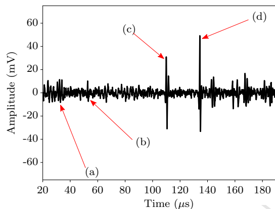
Figure 16: Pulse-echo A-scan data recorded on a 32 cm thick steel sample with a 6 mm diameter side-drilled hole at a depth of 16 cm (see figure 15). The received signals are interpreted as: (a), Rayleigh wave signals reflected from the sample edges at the surface, (b), back-scattered longitudinal wave from the defect, (c), reflected longitudinal wave from the sample's backwall, (d), reflected longitudinal wave from the back wall that has mode-converted at the defect and forward-scattered as a shear wave.
