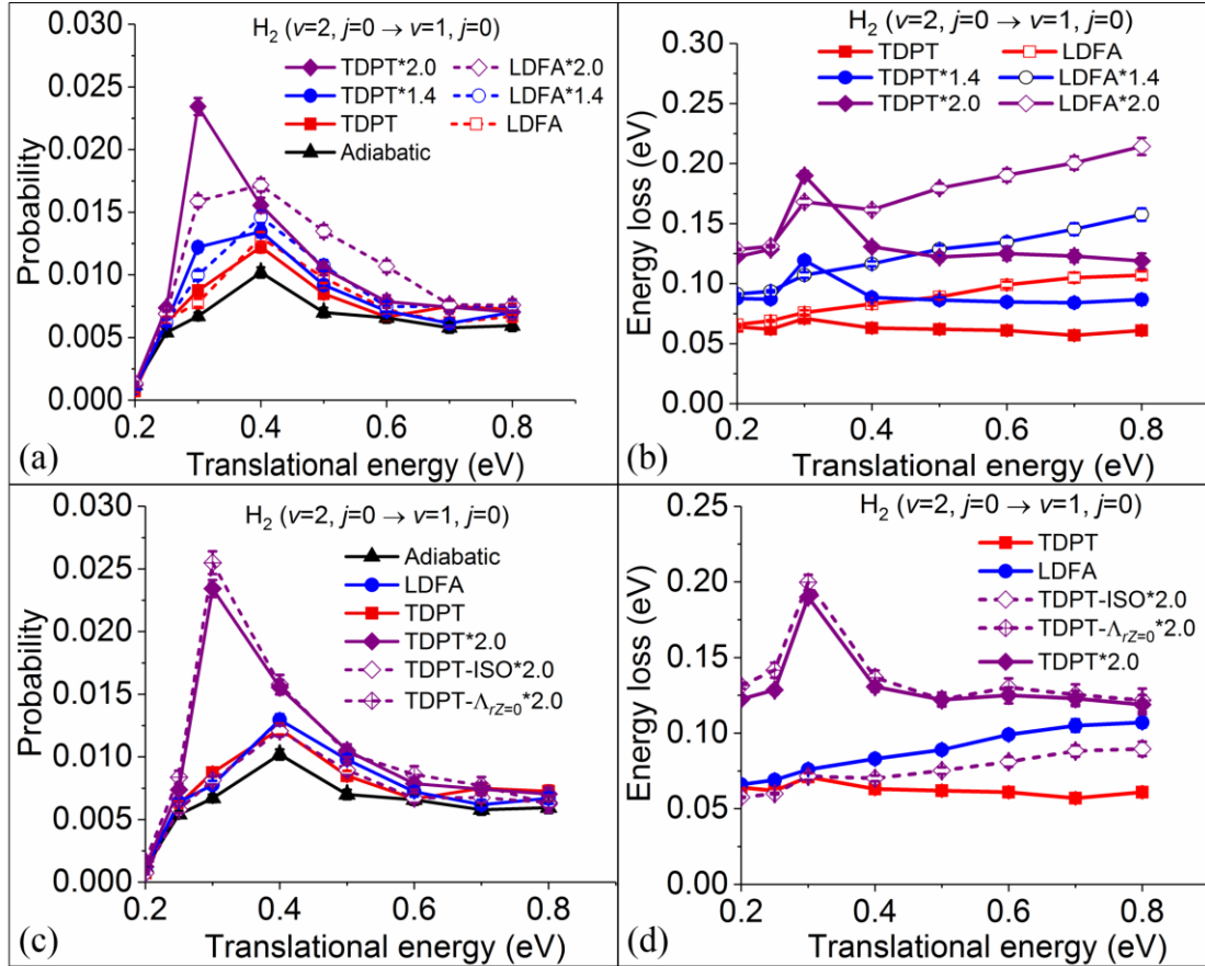
Figure 4. (a) Vibrational deexcitation probabilities from H_2(v=2, j=0) to H_2(v=1, j=0) as a function of translational energy, with adiabatic dynamics (triangles), with electronic friction by LDFA (open symbols) and TDPT (solid symbols) models, and with 1.4 (circles) and 2.0 (diamonds) times larger friction coefficients. (b) Mean nonadiabatic energy losses for various simulations in panel (a). (c) On the basis of (a) but adding new data computed by removing anisotropy (TDPT-ISO*2) and Z - r coupling term (TDPT- \Lambda_{rZ=0} *2.0) in the TDPT friction tensor. (d). Mean nonadiabatic energy losses for various simulations in panel (b).
