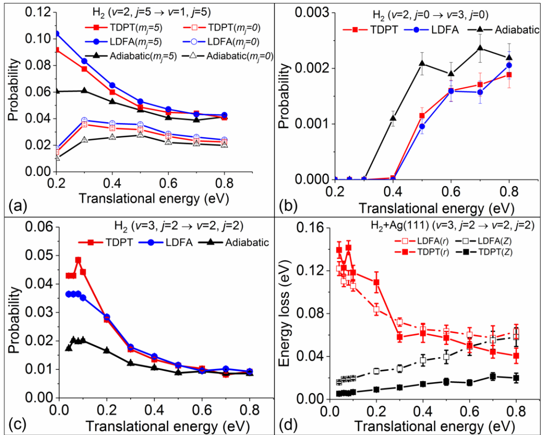
Figure 5. (a) Vibrational state-to-state deexcitation probabilities from H 2 ( v=2, j=5 ) to H 2 ( v=1, j=5 ) for rotationally excited initial conditions as predicted with MD, MDEF(LDFA), and MDEF(TDPT). (b) Vibrational excitation probabilities upon scattering (c) Vibrational deexcitation probability from H 2 ( v=3, j=2 ) to H 2 ( v=2, j=2 ). (d) Energy loss for during vibrational deexcitation from H 2 ( v=3, j=2 ) to H 2 ( v=2, j=2 ).
