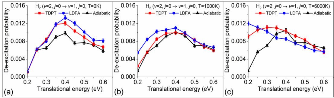
Figure 7. Vibrational deexcitation probabilities from H_2(v=2, j=0) to H_2(v=1, j=0) simulated by MD, MDEF(LDFA), and MDEF(TDPT), with electronic temperature of 0 K (a), 1000 K (b), and 6000 K (c).
