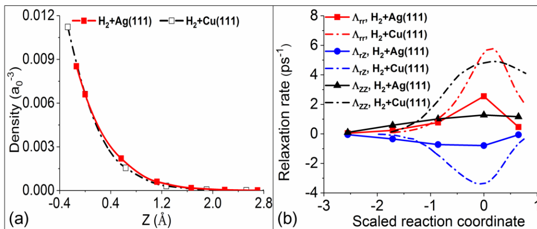
Figure 3a. (a) Comparison of the clean metal substrate electron density evaluated at the position of an H atom moving along the MEPs for dissociation on Cu(111) and Ag(111), as a function of the relative height with respect to the molecular center at the transition state ( i.e. Z_{\text{TS}}=0 ). (b) Comparison of the mode-specific electronic friction computed by TDPT along the MEPs for \text{H}_2 dissociation on Cu(111) and Ag(111).
