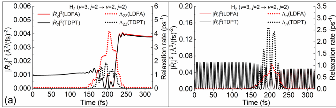
Figure 6. Variation of the square of velocity (solid lines) in Z ( |\dot{R}_z|^2 , panel a) and r ( |\dot{R}_r|^2 , panel b) directions along with the corresponding friction coefficients (dotted lines), as a function of time for a representative trajectory for \text{H}_2(v=3, j=2) to \text{H}_2(v=2, j=2) scattering on \text{Ag}(111) , at translational energy of 0.1 eV.
