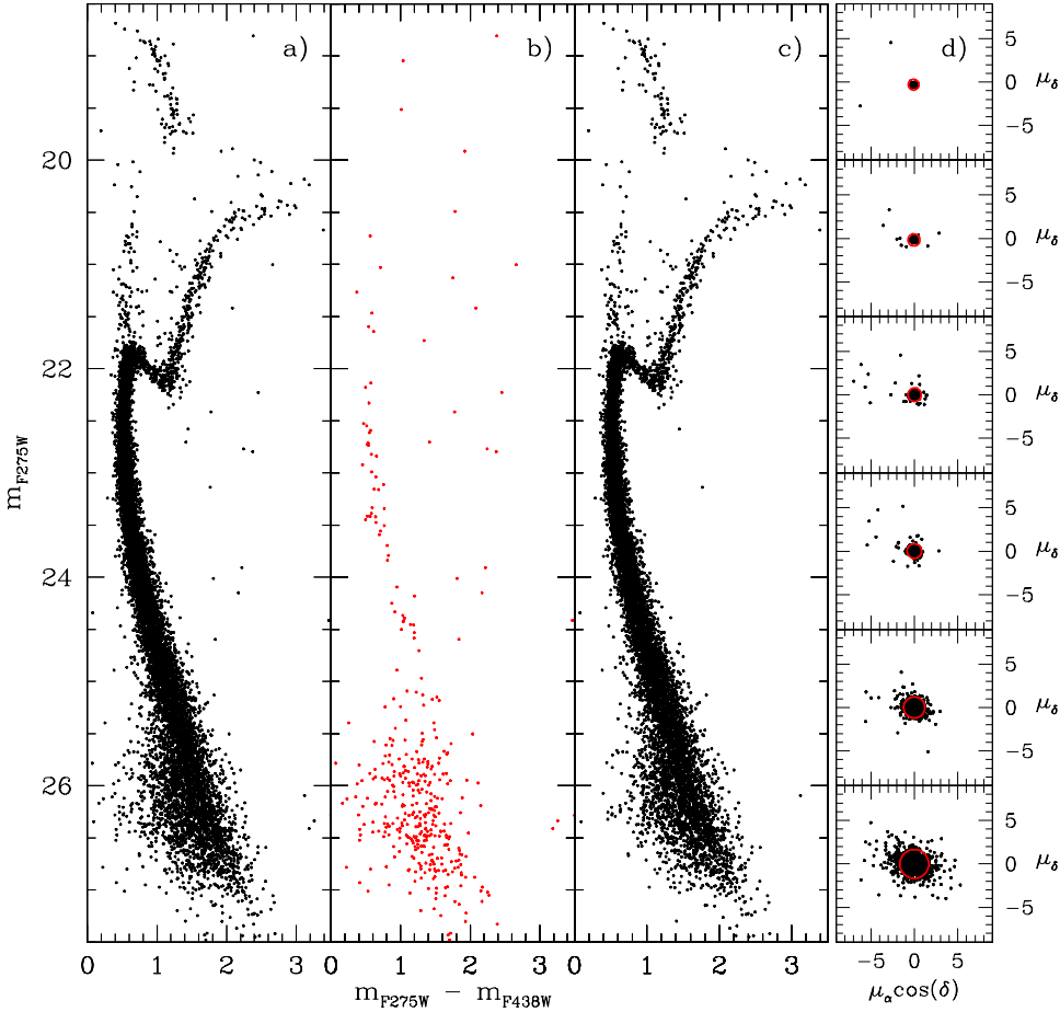
Fig. 2. Panel a: ( m_{F275W} , m_{F275W} - m_{F438W} ) CMD of all the stars in common between the ACS and WFC3 catalogues; panel b: CMD of all the likely contaminating objects as selected from the VPDs; panel c: relative PM-cleaned CMD obtained by using only likely cluster members; panels d: VPDs at different magnitude levels. The solid red circle represents the fiducial region used to select likely cluster members.
