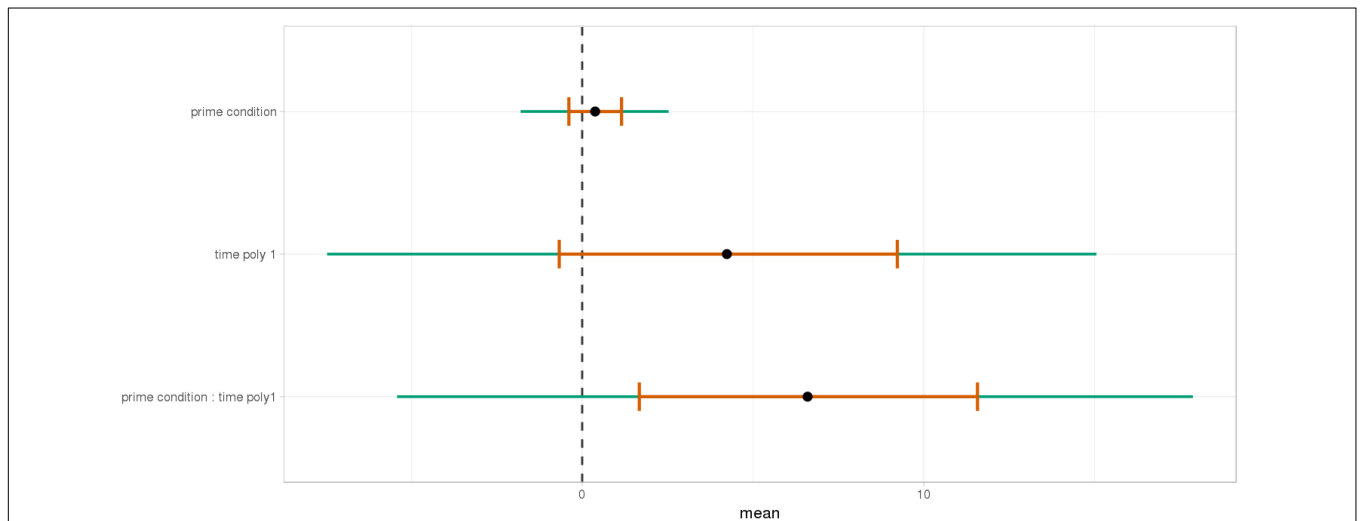
FIGURE 13 | Posterior distribution of independent variables for the first part (1062–1462 ms) in the mathematical knowledge group.
