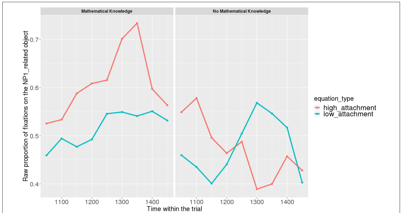
FIGURE 12 | Proportions of looks toward the NP1-related object in each of the two groups at the beginning of the relative clause (1063–1463 ms). Red curves: high-attachment prime condition; blue curves: low-attachment prime condition (Items variable).
