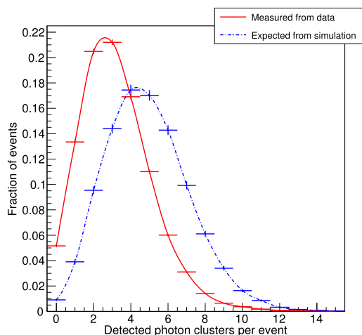
Fig. 18. Measured photon counting statistics per event in 2016 testbeam data (red) and expected from simulation (blue). (For interpretation of the references to colour in this figure legend, the reader is referred to the web version of this article.)
