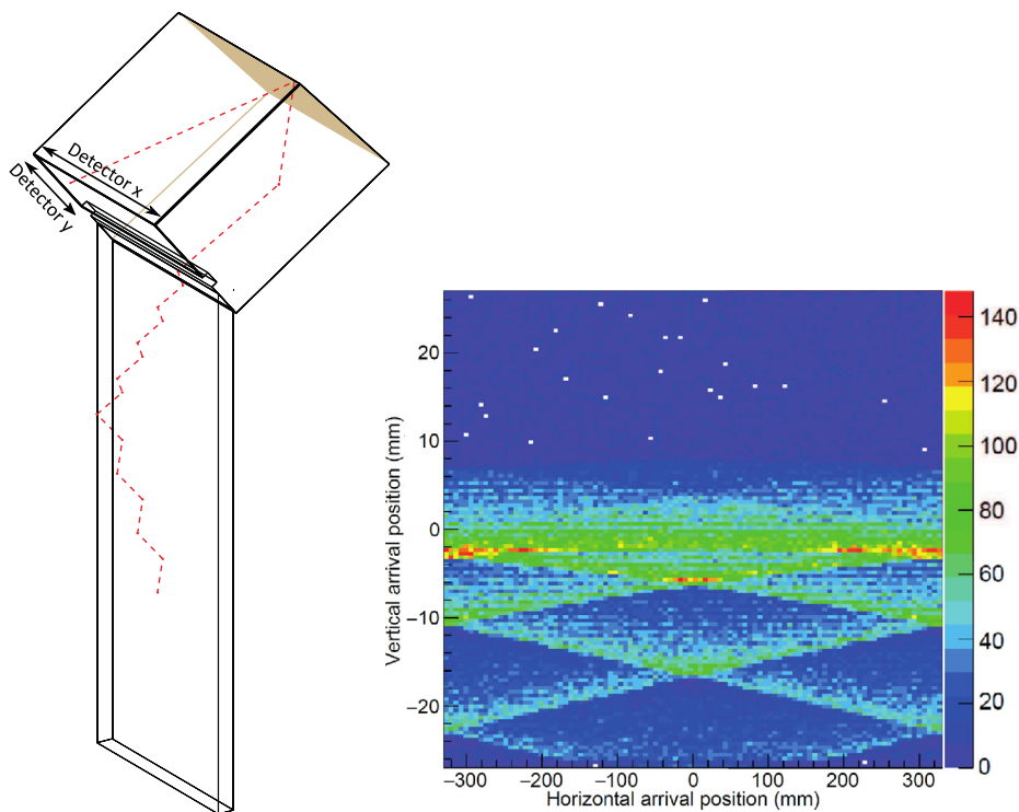
Fig. 5. (Left) Isometric view of a TORCH module of reduced size showing the path of a single photon propagating through the optics (red dashed line) and showing the definition of horizontal ( x_{detector} ) and vertical direction ( y_{detector} ); (Right) the folded pattern of photons expected to arrive at the photodetector plane for a full-sized TORCH module, derived from GEANT simulation. (For interpretation of the references to colour in this figure legend, the reader is referred to the web version of this article.)
